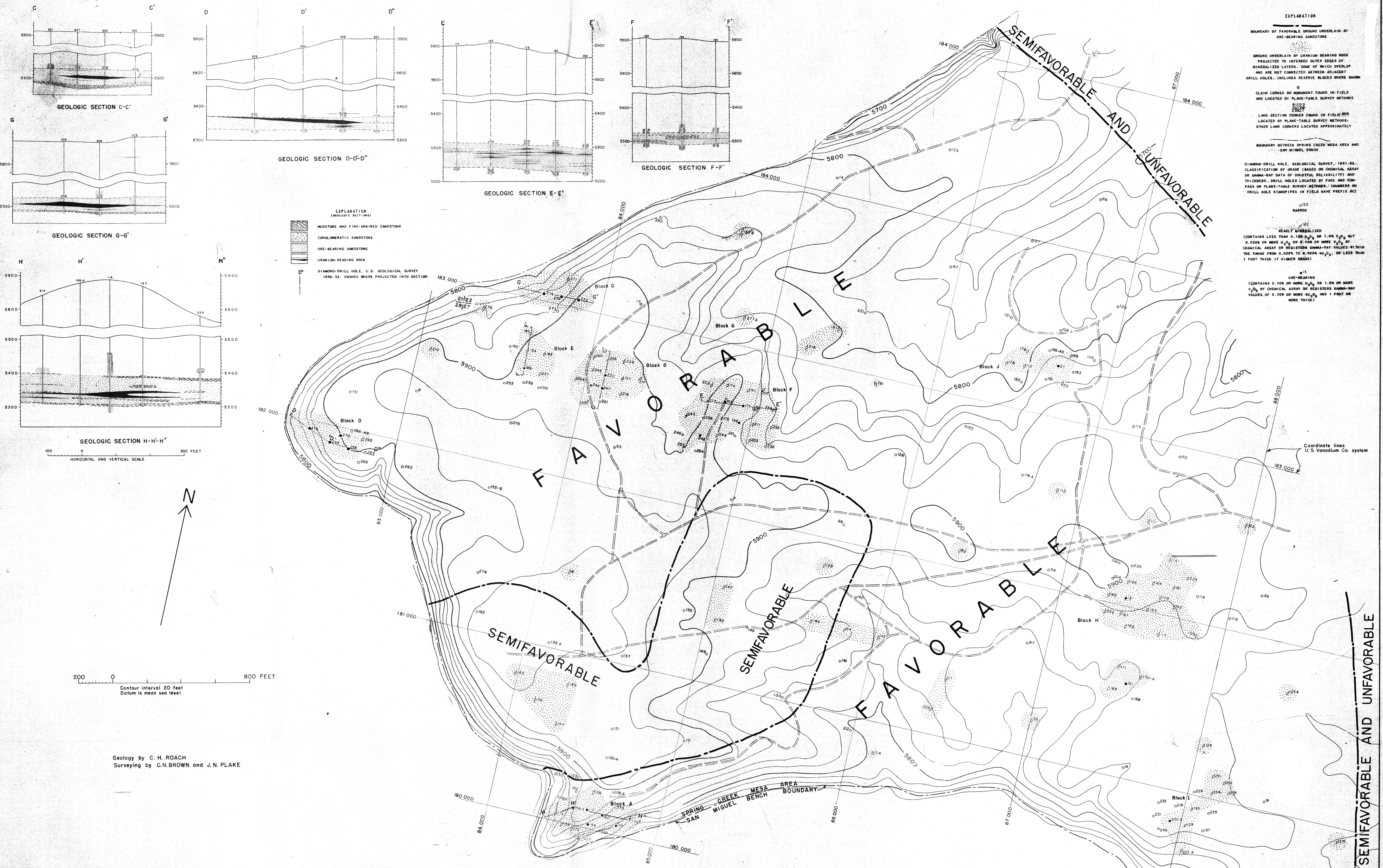
Figure 3. GEOLOGIC MAP AND SECTIONS OF THE WESTERN PART OF SPRING CREEK MESA, MONTROSE COUNTY, COLORADO
