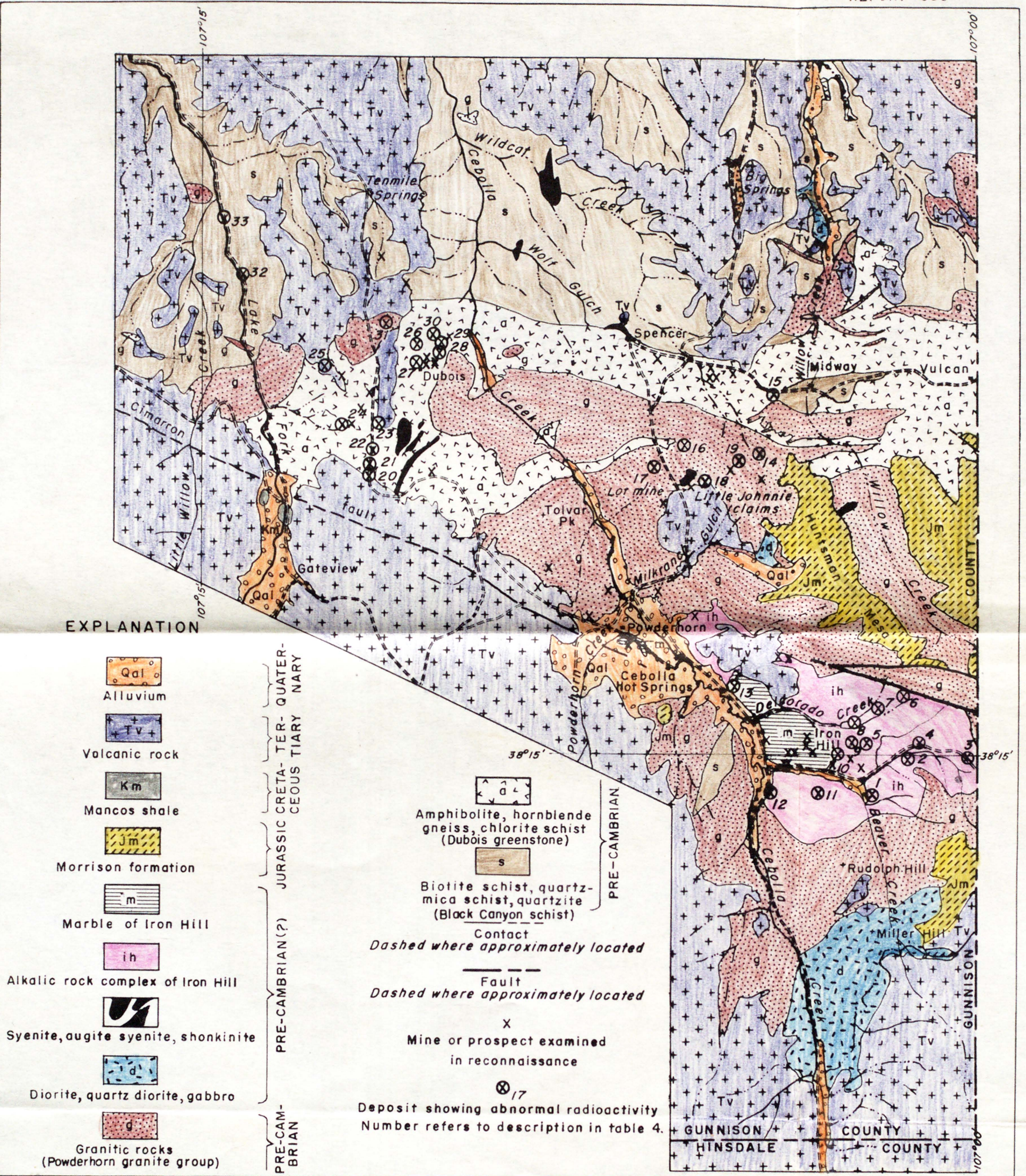
FIGURE 2.—GENERALIZED GEOLOGIC MAP OF THE POWDERHORN DISTRICT, COLORADO, SHOWING LOCALITIES EXAMINED
