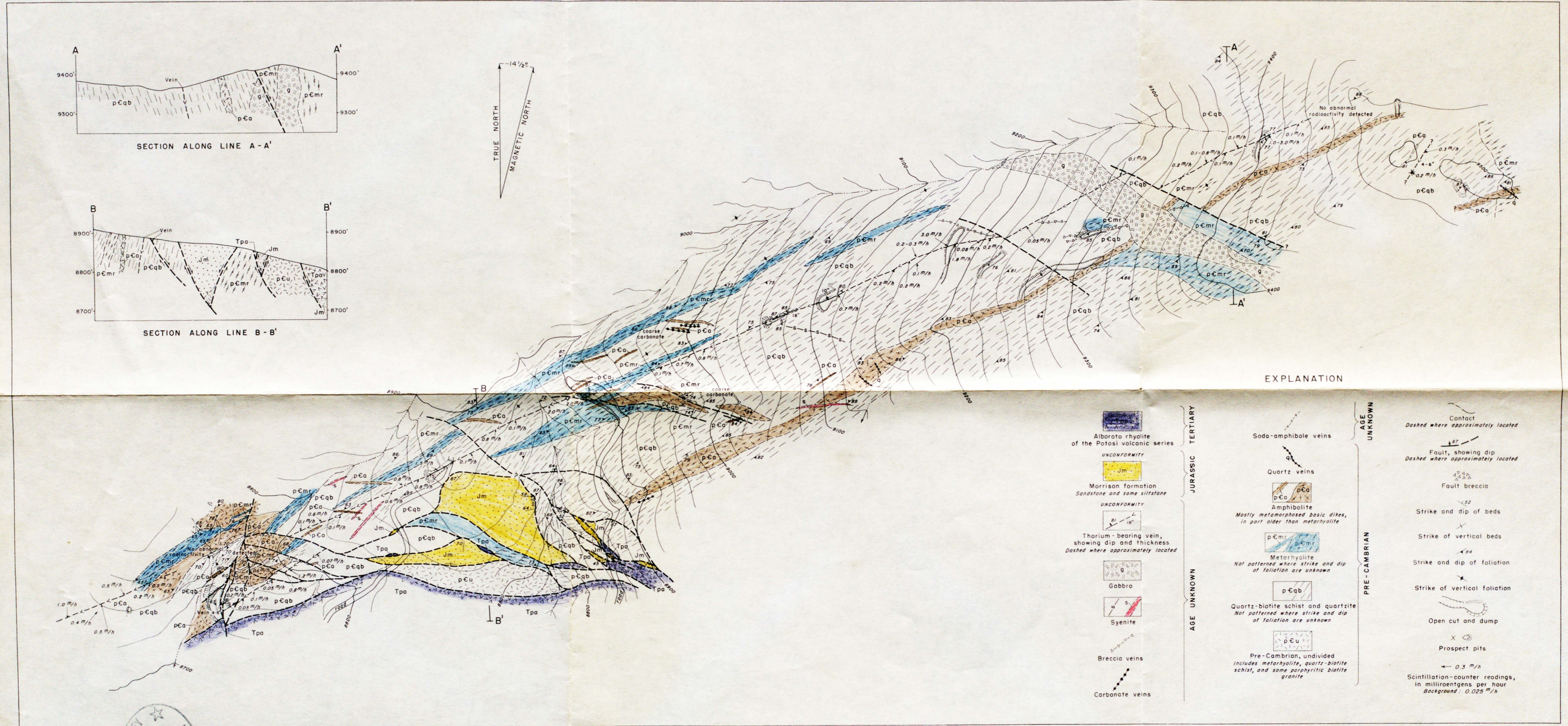
FIGURE 3. — GEOLOGIC MAP AND SECTIONS OF THE LITTLE JOHNNIE THORIUM DEPOSIT, GUNNISON COUNTY, COLORADO
