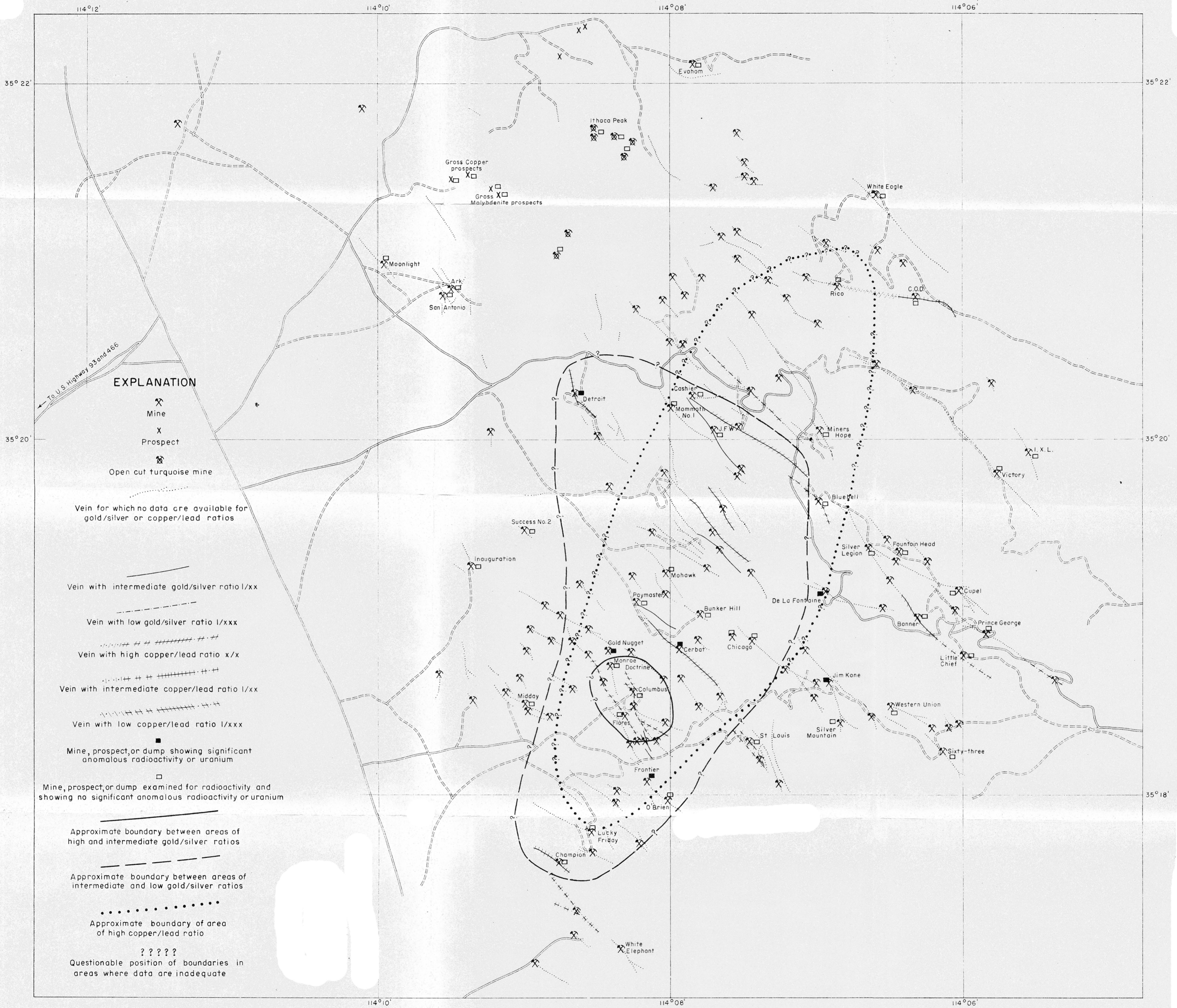
FIGURE 2.—MAP SHOWING ZONAL DISTRIBUTION OF METAL RATIOS AND RESULTS OF RADIOACTIVITY RECONNAISSANCE IN THE SOUTHERN PART OF THE WALLAPAI MINING DISTRICT, MOHAVE COUNTY, ARIZONA
