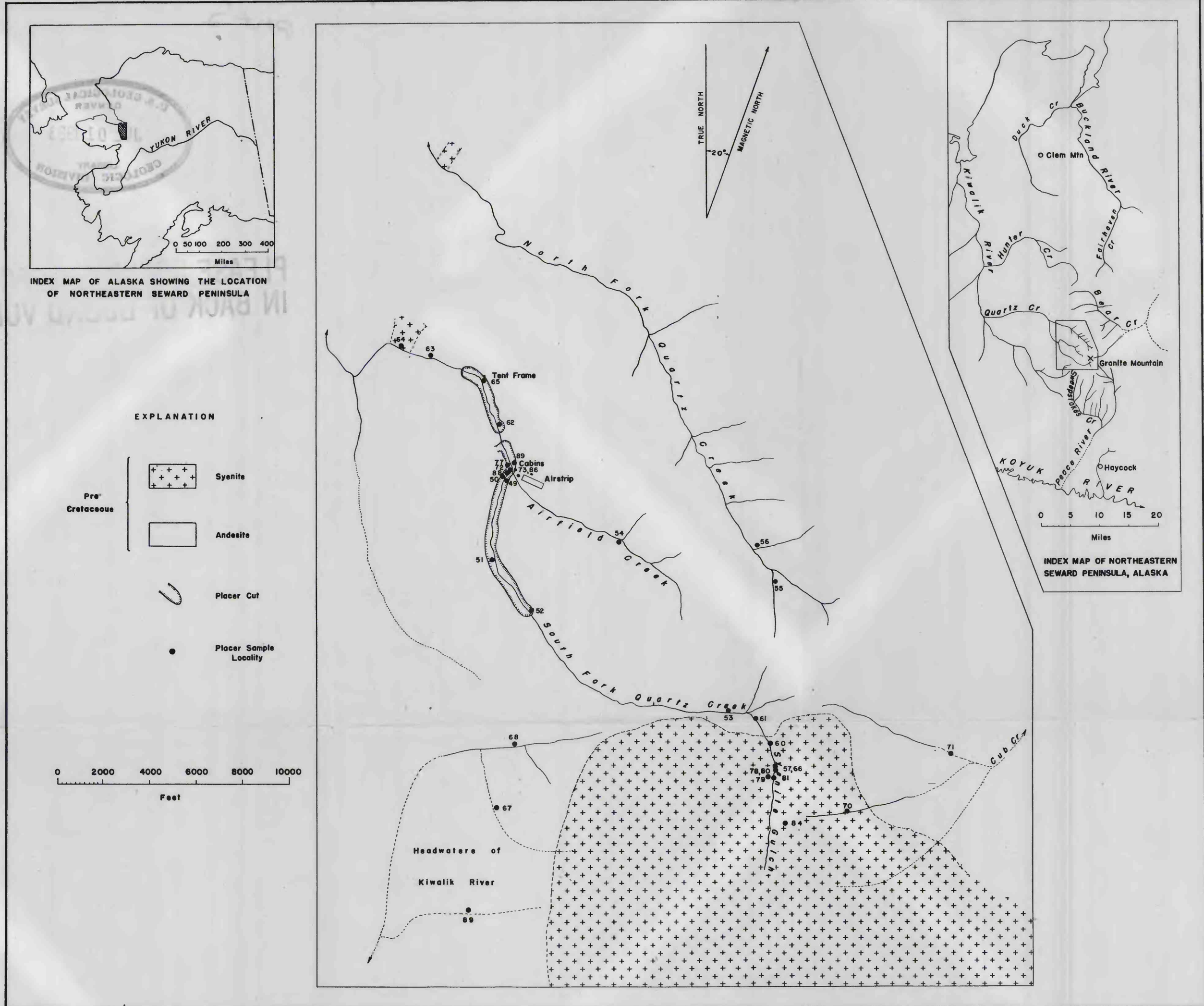
FIGURE 1- GEOLOGIC SKETCH MAP OF THE UPPER PORTION OF QUARTZ CREEK, NORTHEASTERN SEWARD PENINSULA, ALASKA
