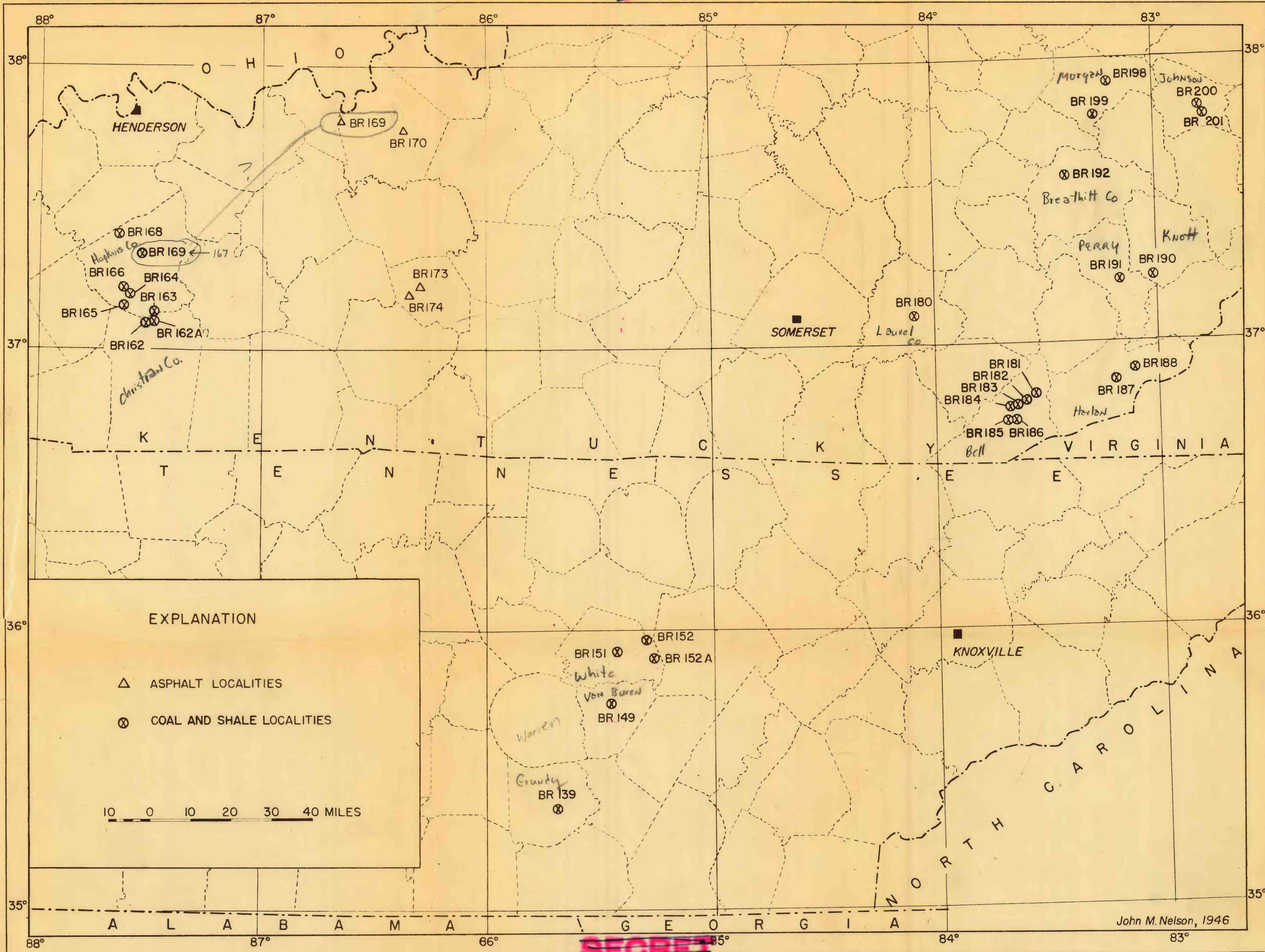
INDEX MAP OF ASPHALT, COAL, AND SHALE LOCALITIES IN TENNESSEE AND KENTUCKY
