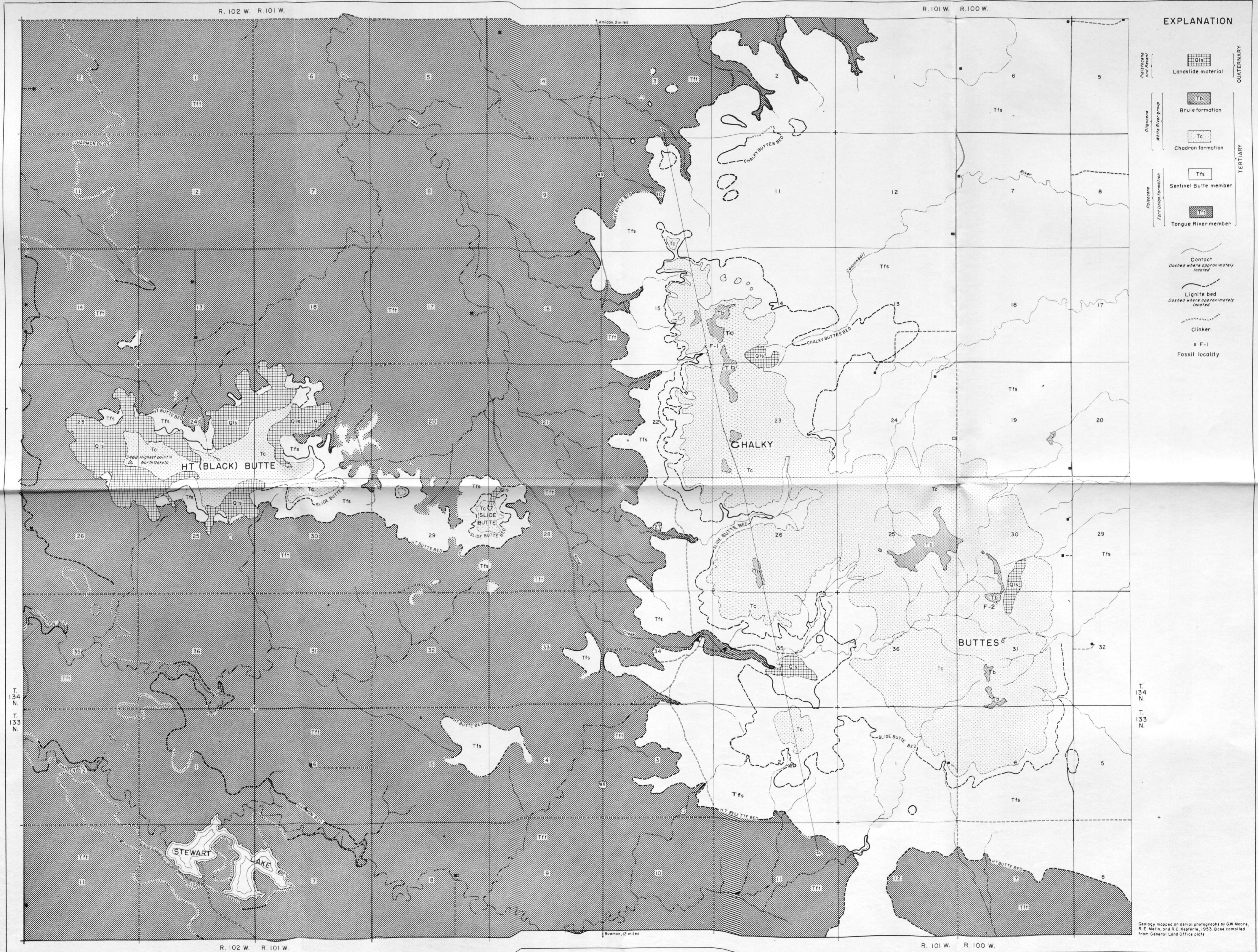
FIGURE 7 —GEOLOGIC MAP OF THE CHALKY BUTTES AREA, SLOPE COUNTY, NORTH DAKOTA
