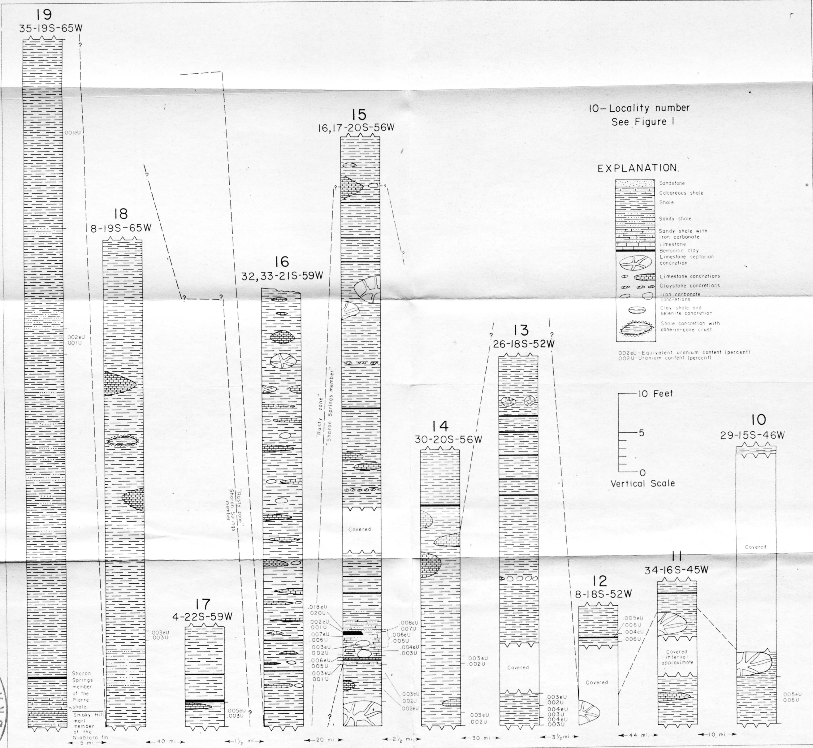
FIGURE 3—GRAPHIC SECTIONS OF LOWER PART OF PIERRE SHALE IN CHEYENNE, KIOWA, CROWLEY, AND PUEBLO COUNTIES, COLORADO
