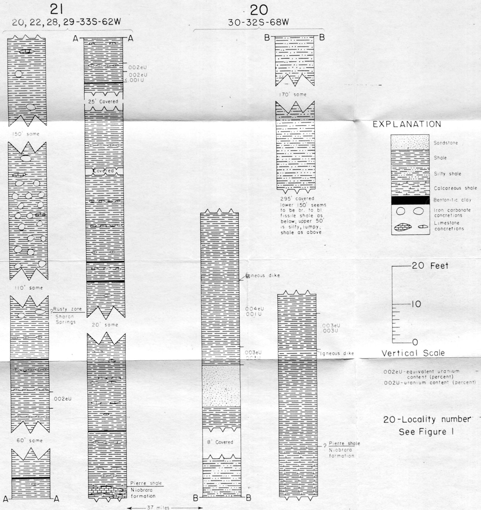
FIGURE 4-GRAPHIC SECTIONS OF LOWER PART OF PIERRE SHALE IN LAS ANIMAS COUNTY, COLORADO.
