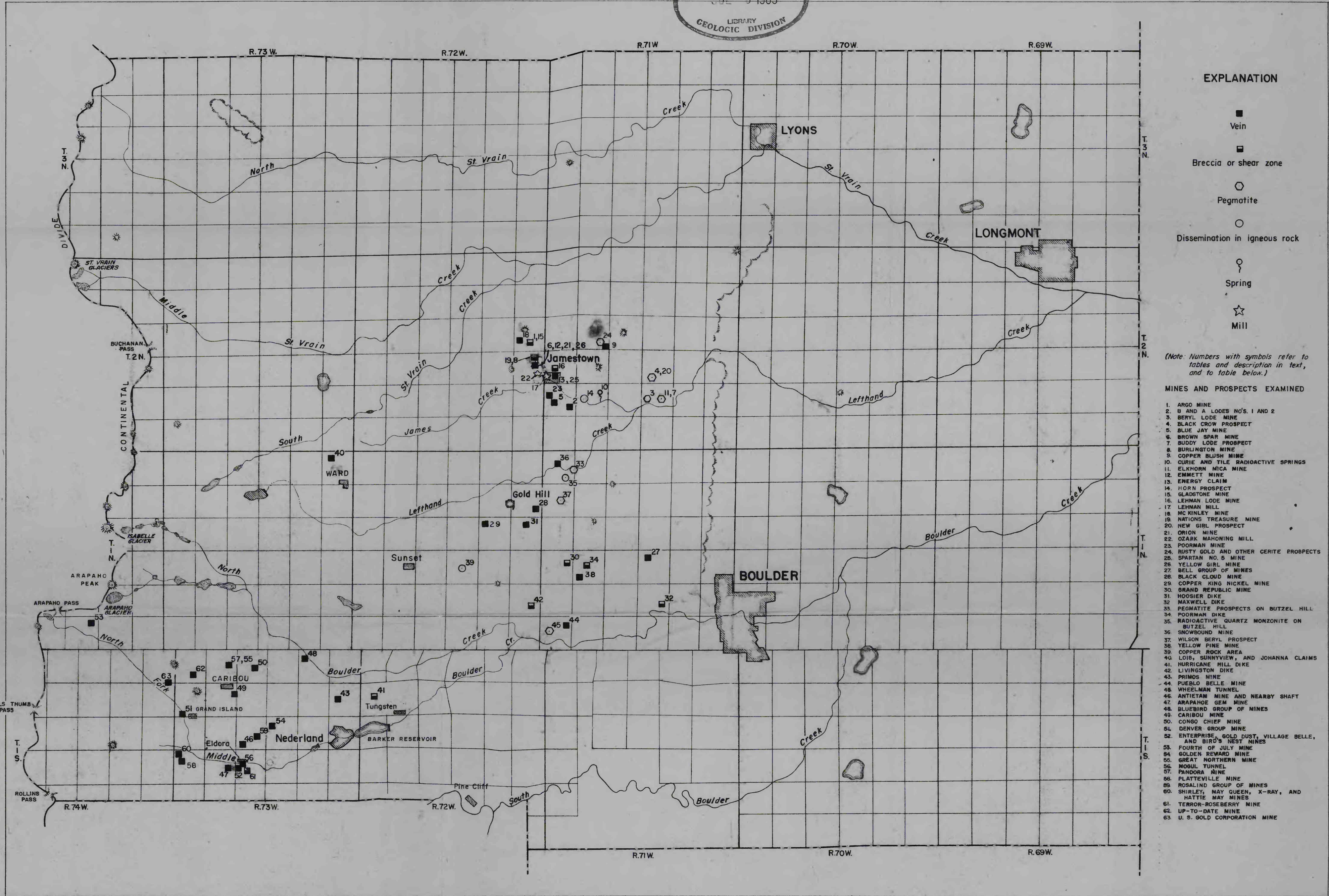
FIGURE 2 . - INDEX MAP SHOWING LOCATION OF URANIUM DEPOSITS IN BOULDER COUNTY, COLORADO
