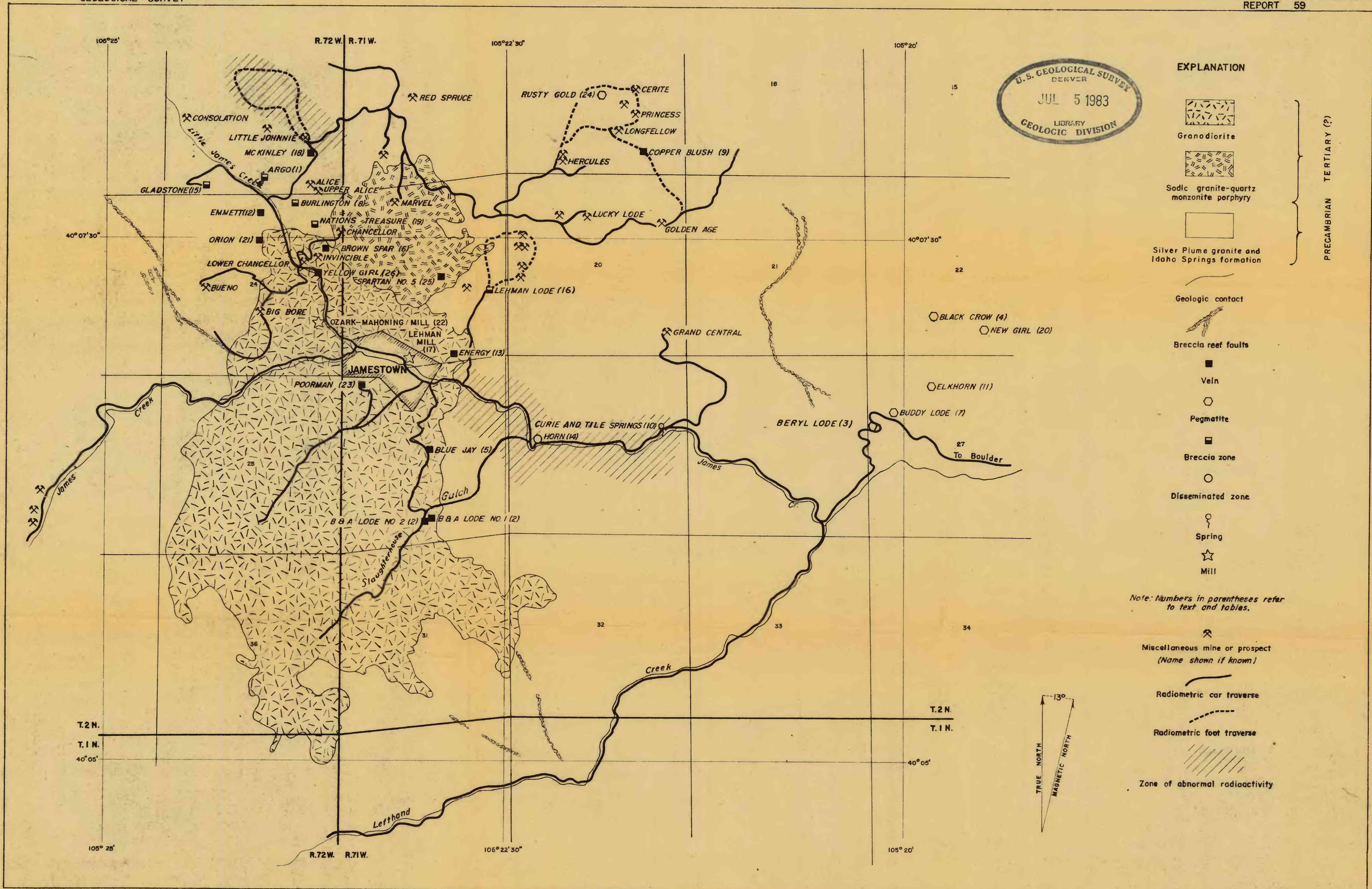
FIGURE 3. - MAP OF THE JAMESTOWN DISTRICT, SHOWING LOCALITIES EXAMINED FOR URANIUM
