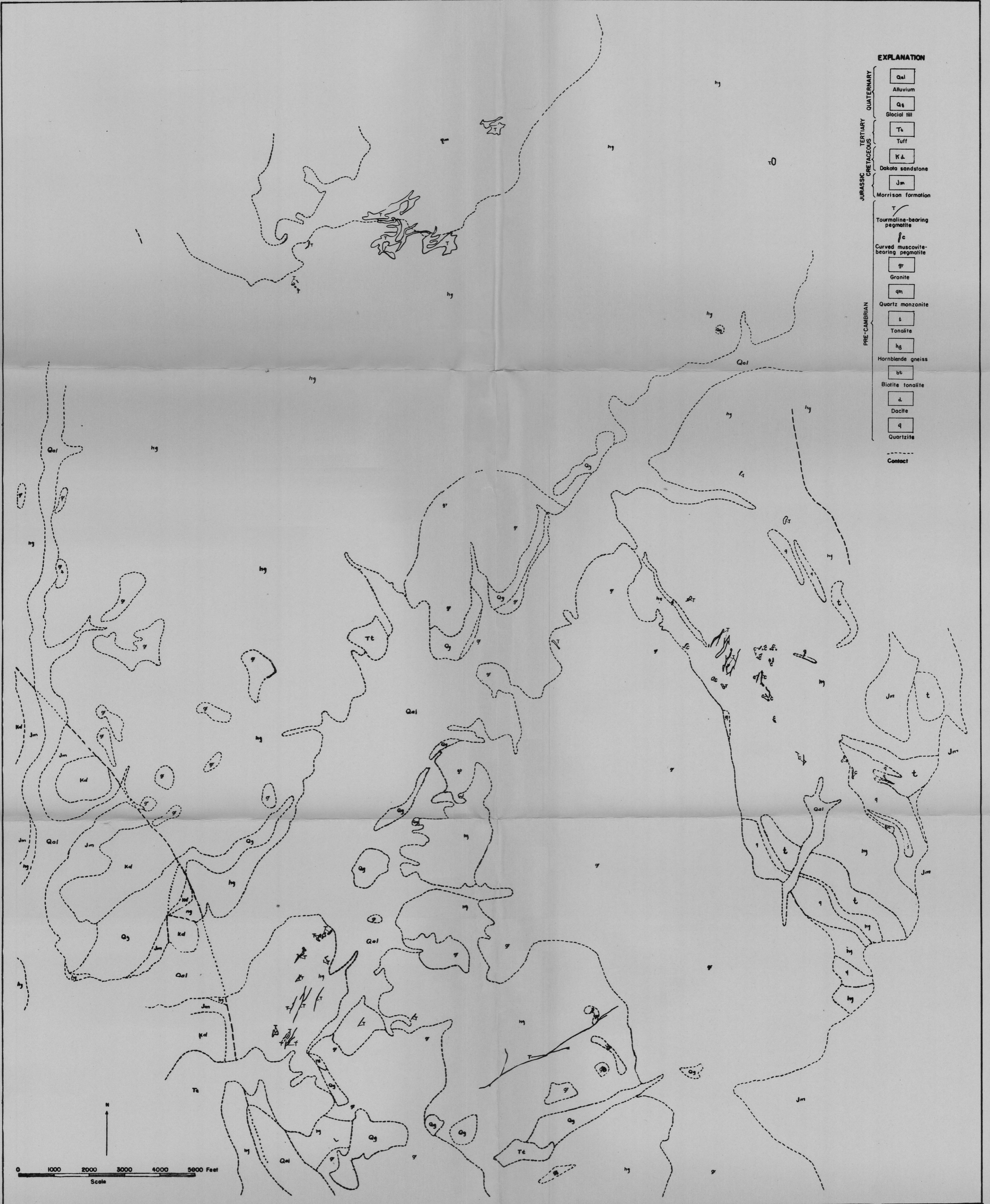
FIGURE 17. DISTRIBUTION OF TOURMALINE- AND CURVED MUSCOVITE-BEARING PEGMATITES
