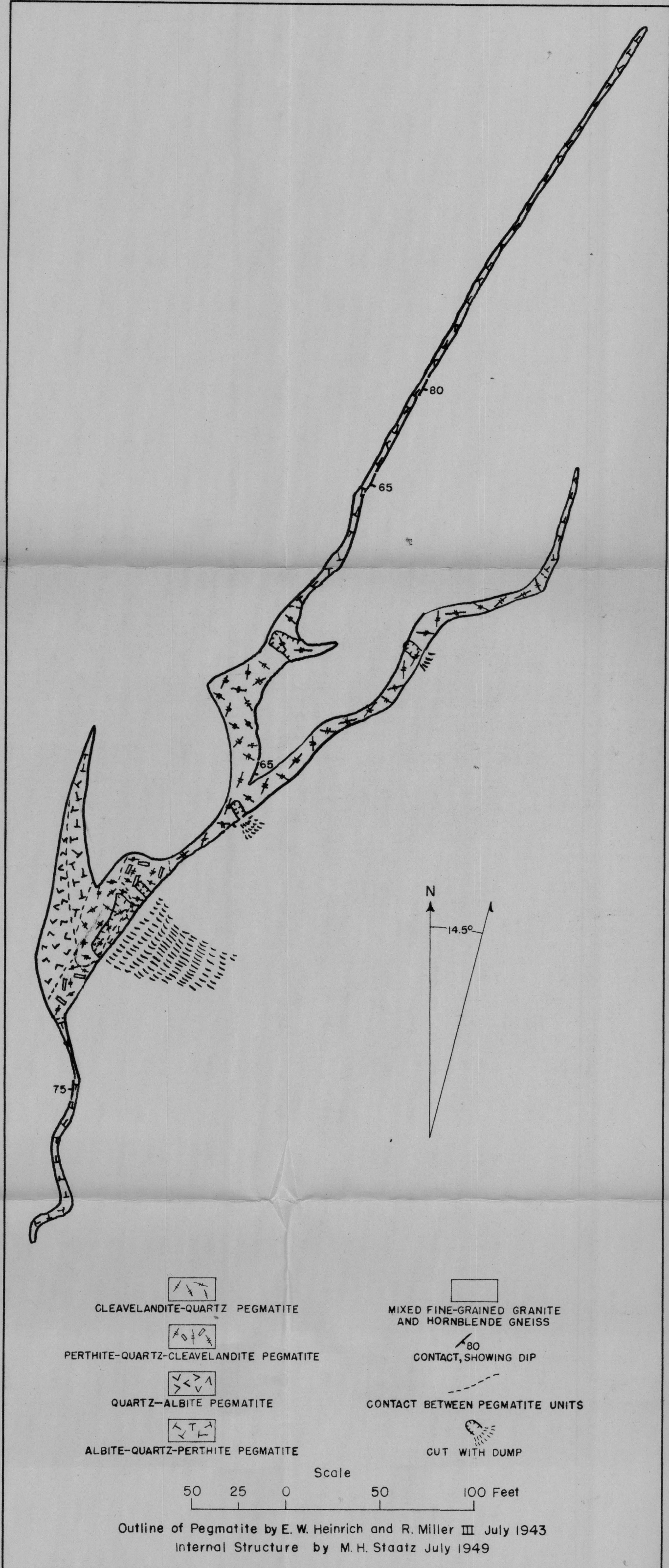
FIGURE 21. GEOLOGIC MAP, OPPORTUNITY NO. 1 (NO. 215) PEGMATITE
