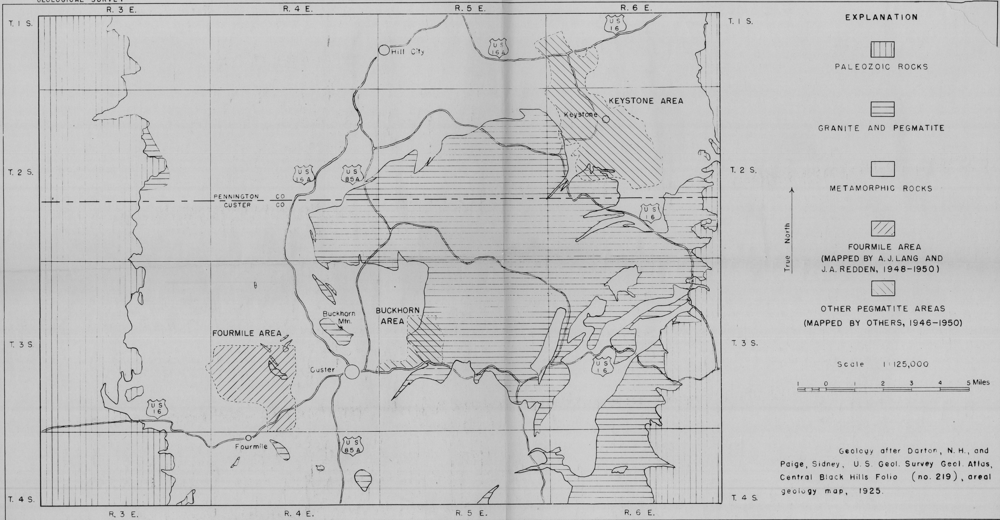
FIGURE 1. MAP OF THE SOUTHERN BLACK HILLS, SOUTH DAKOTA, SHOWING PEGMATITE AREAS MAPPED IN 1946-1950
