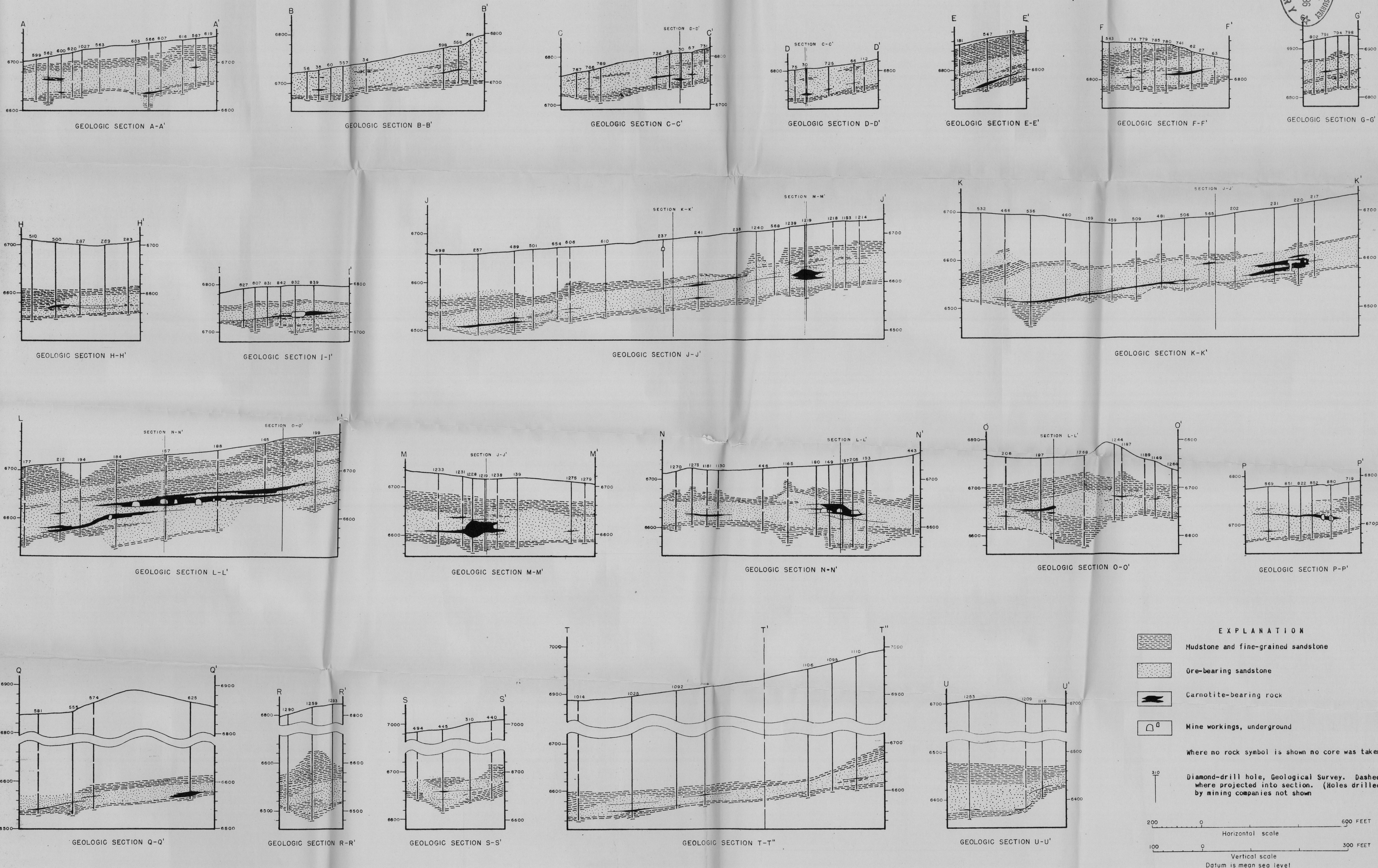
Figure 6-- GEOLOGIC SECTIONS OF OUTLAW MESA, MESA COUNTY, COLORADO
