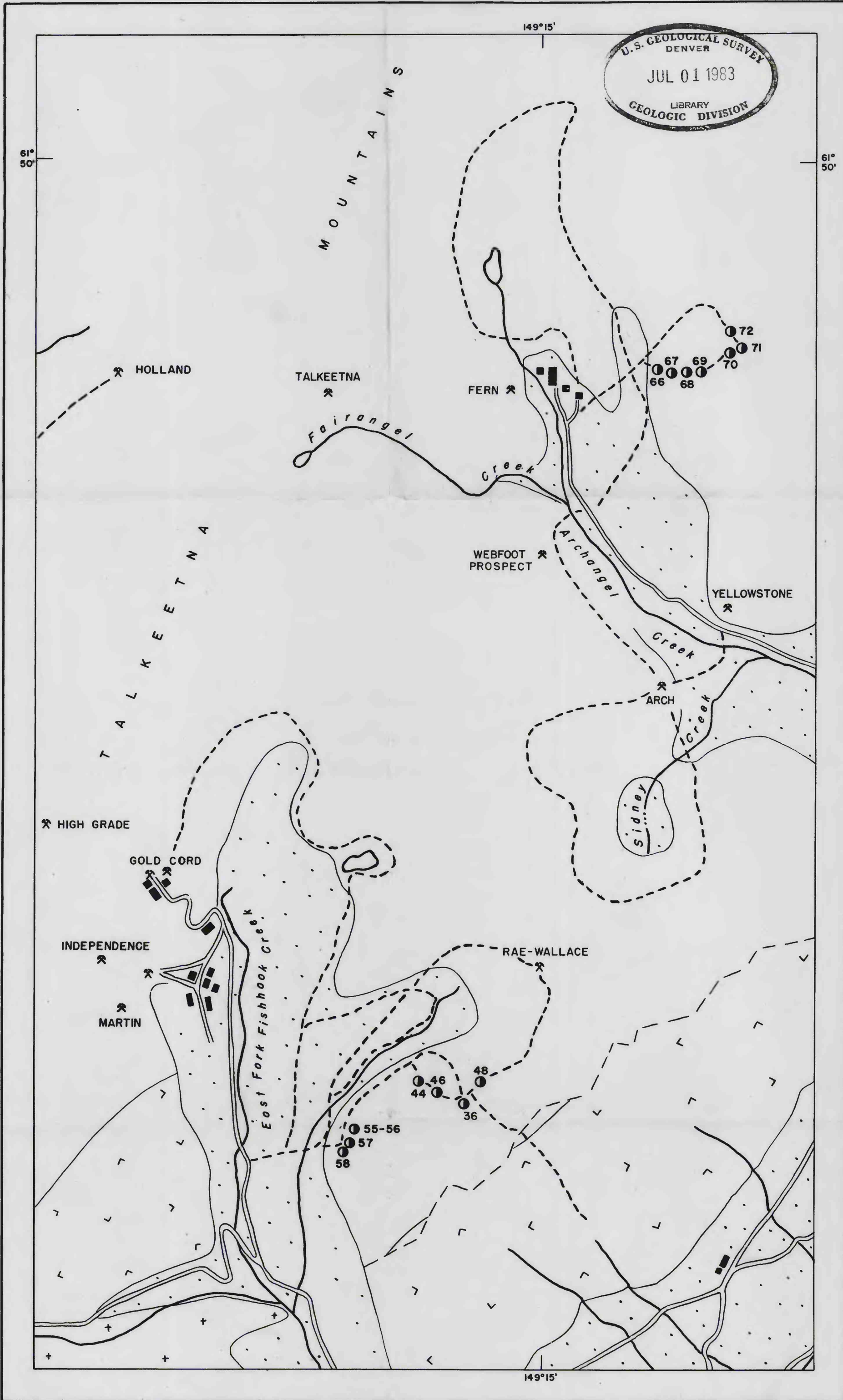
GEOLOGIC MAP OF THE FISHHOOK CREEK-ARCHANGEL CREEK AREA WILLOW CREEK DISTRICT, ALASKA
