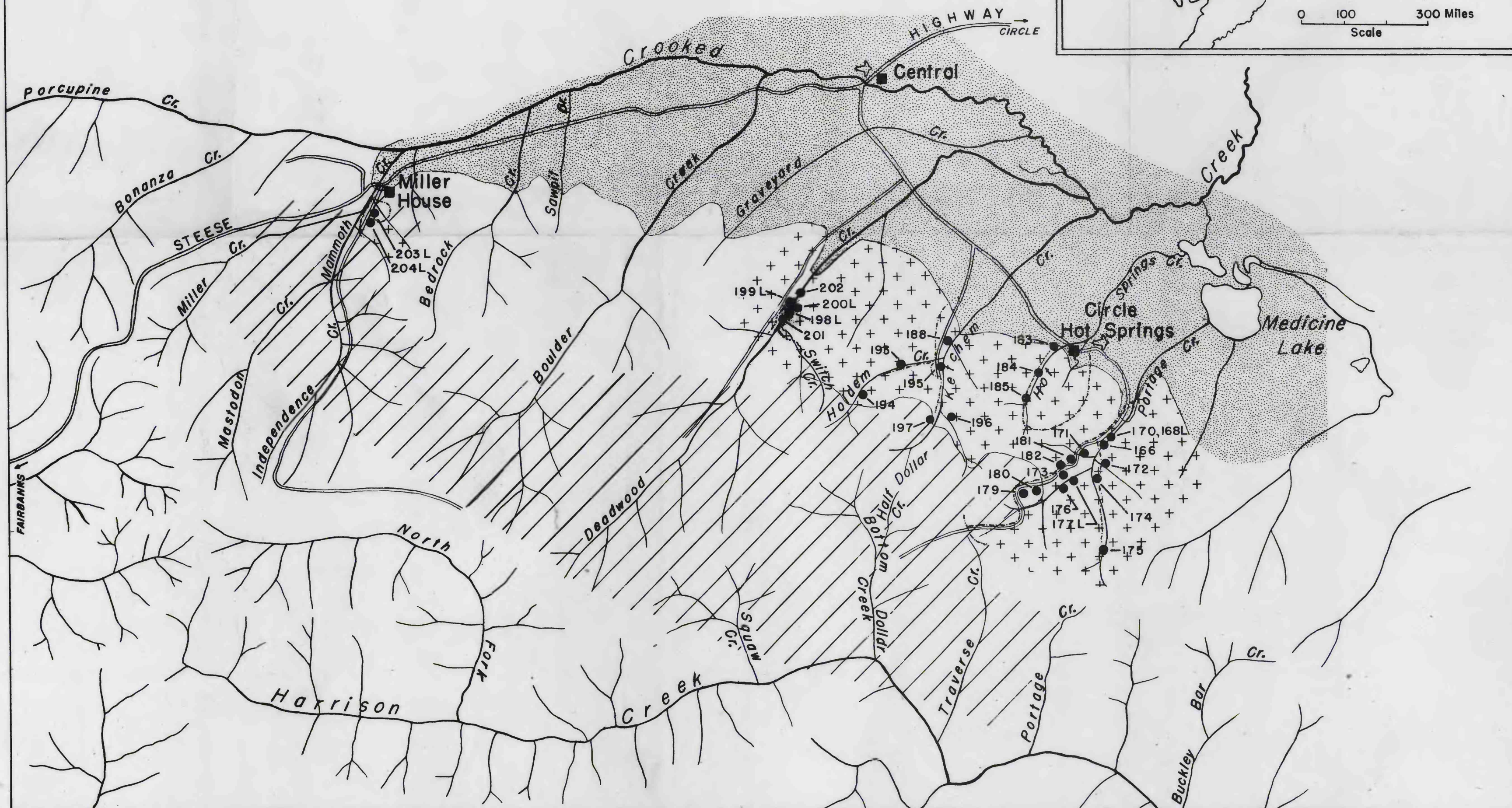
GEOLOGIC SKETCH MAP OF THE MILLER HOUSE - CIRCLE HOT SPRINGS AREA EAST-CENTRAL ALASKA
