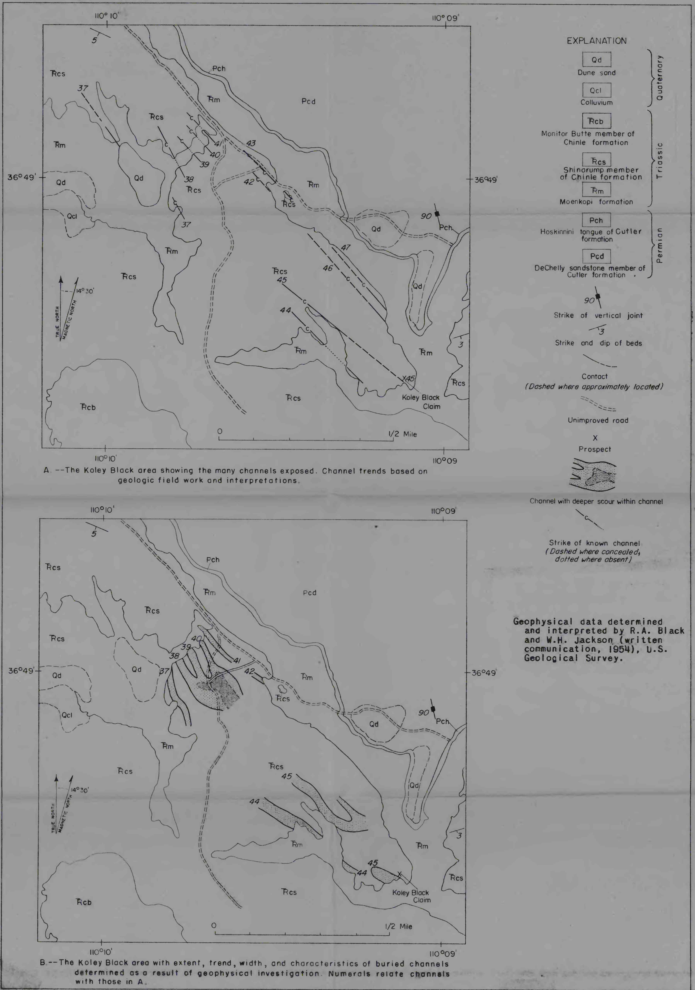
Figure 19.--TWO ILLUSTRATIONS DEMONSTRATING THE USE OF GEOPHYSICAL WORK AS A SUPPLEMENT TO GEOLOGIC MAPPING IN THE SEARCH FOR CHANNELS.
