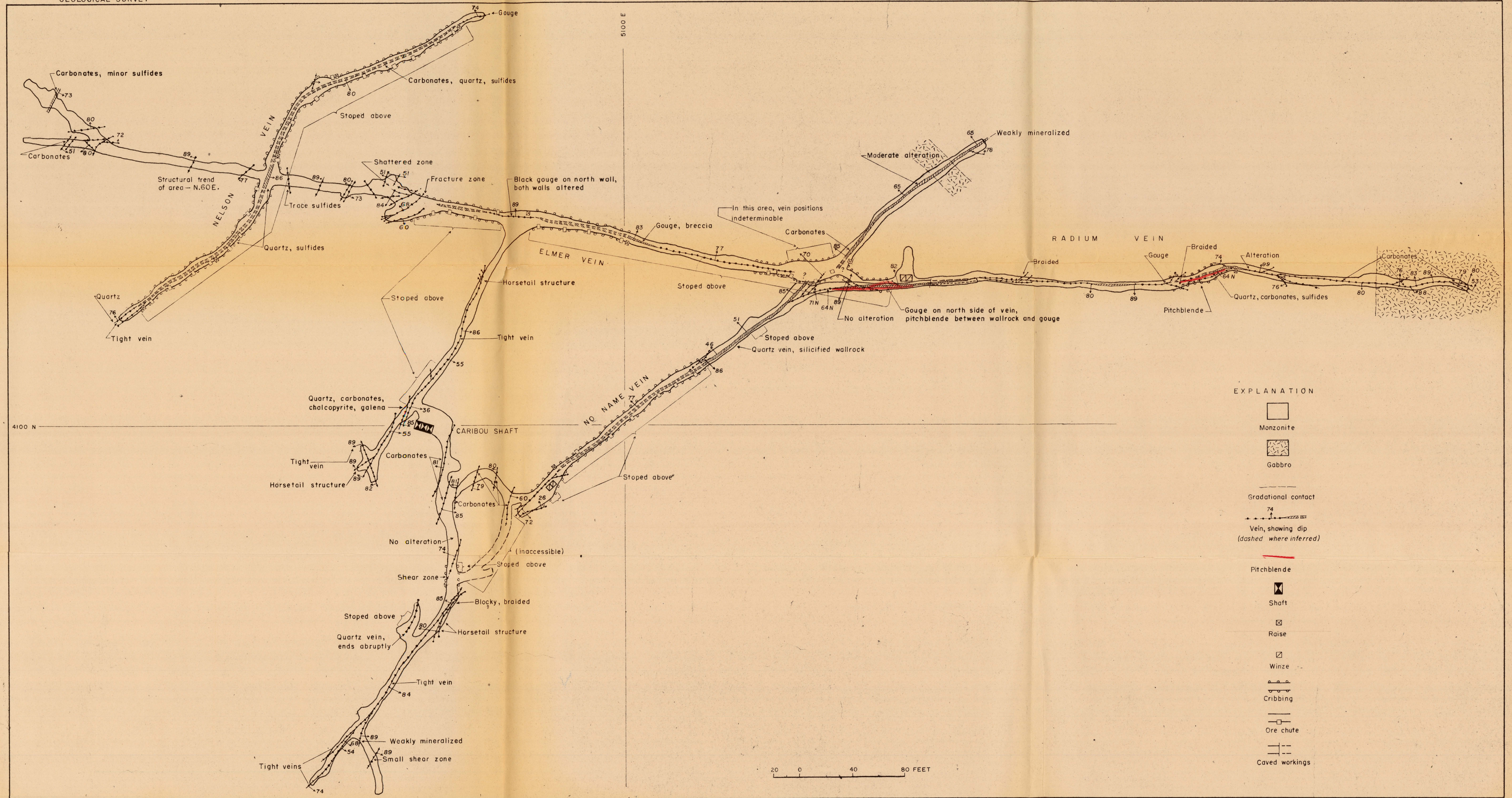
FIGURE 10.—GEOLOGIC MAP OF THE 1040-FOOT LEVEL, CARIBOU MINE, BOULDER COUNTY, COLORADO.
