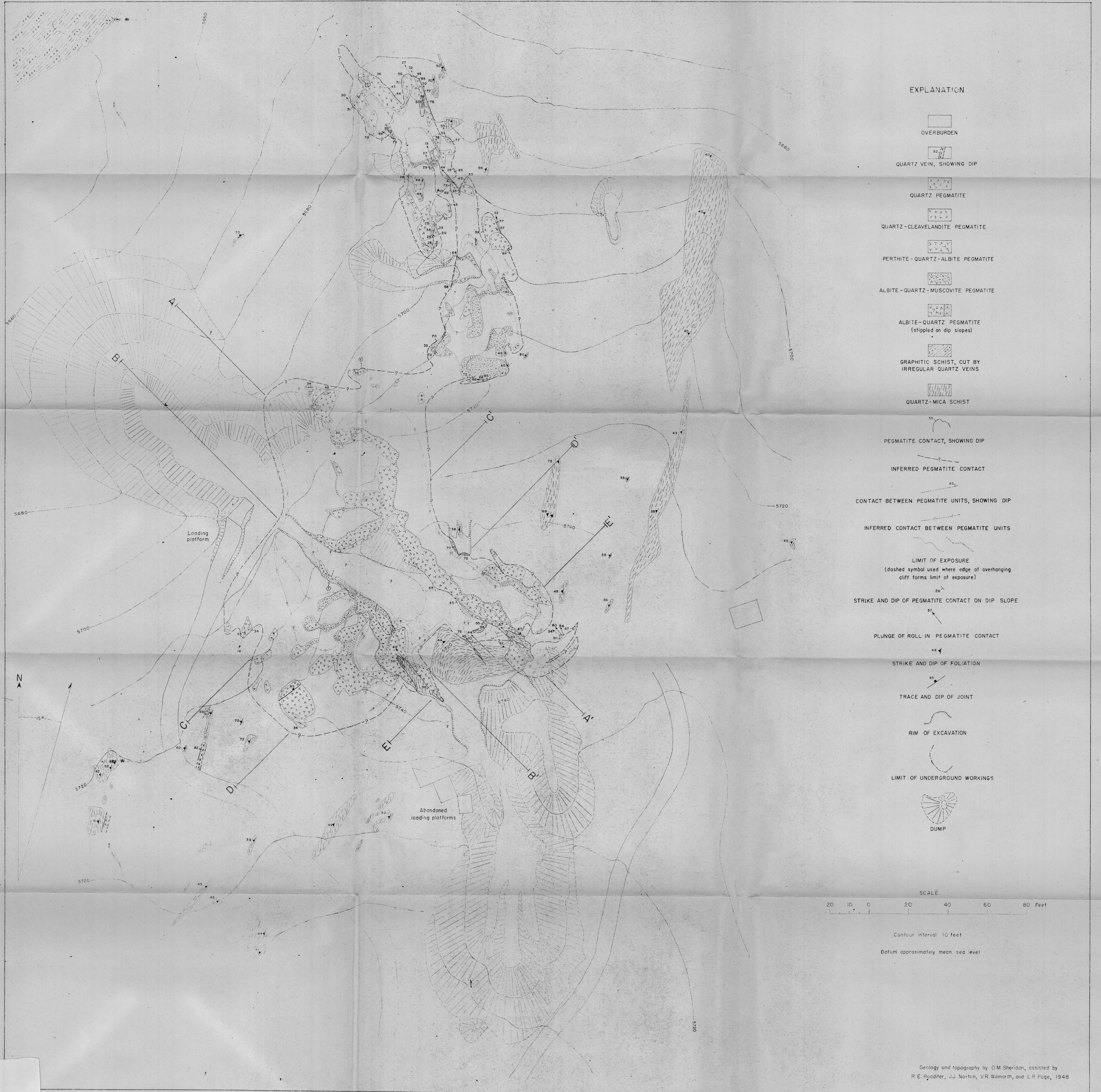
FIGURE 2. GEOLOGIC MAP OF THE HIGH CLIMB PEGMATITE, CUSTER COUNTY, SOUTH DAKOTA
