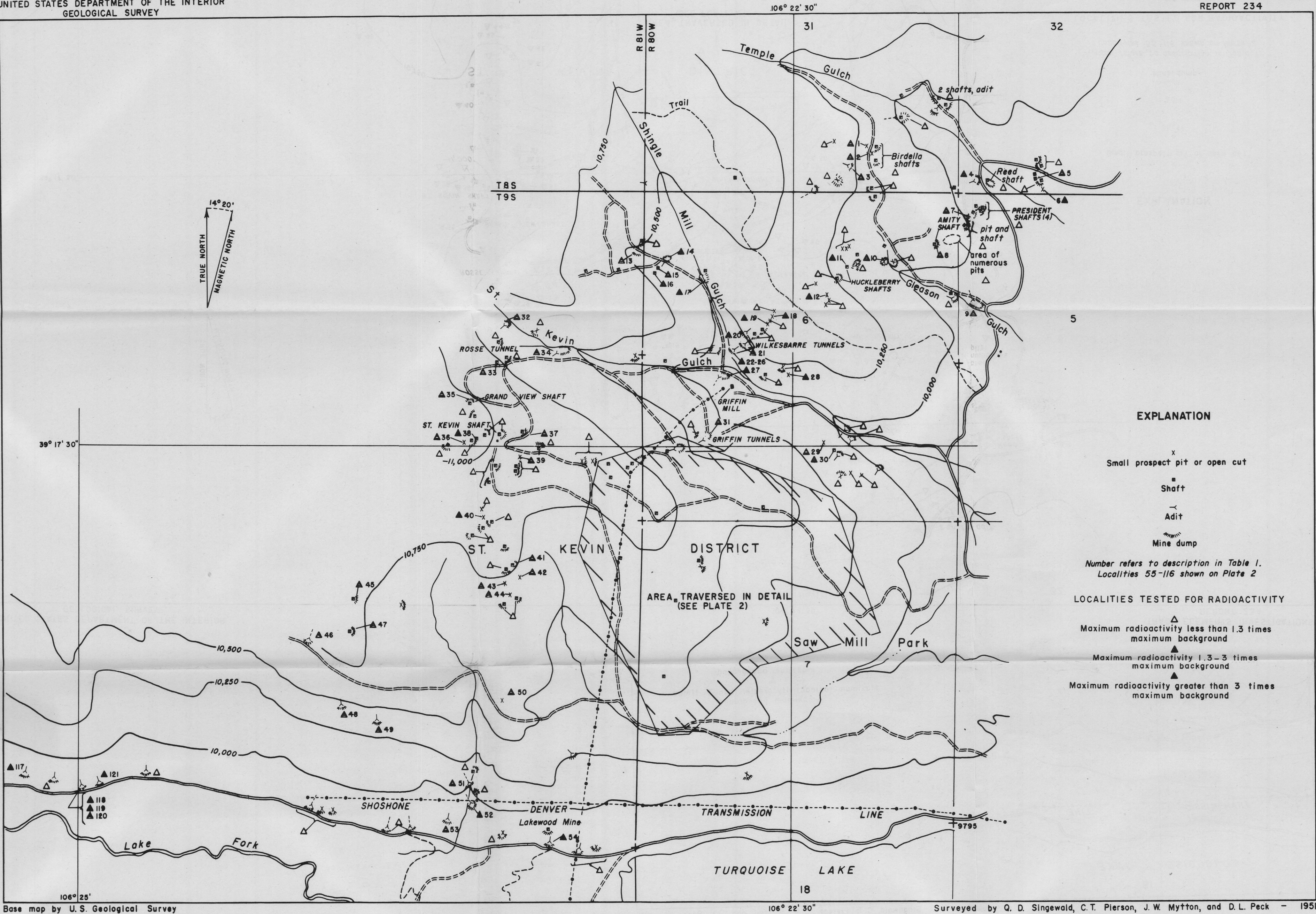
PLATE I.- LOCALITIES TESTED FOR RADIOACTIVITY IN THE ST. KEVIN DISTRICT AND VICINITY, LAKE COUNTY, COLORADO
