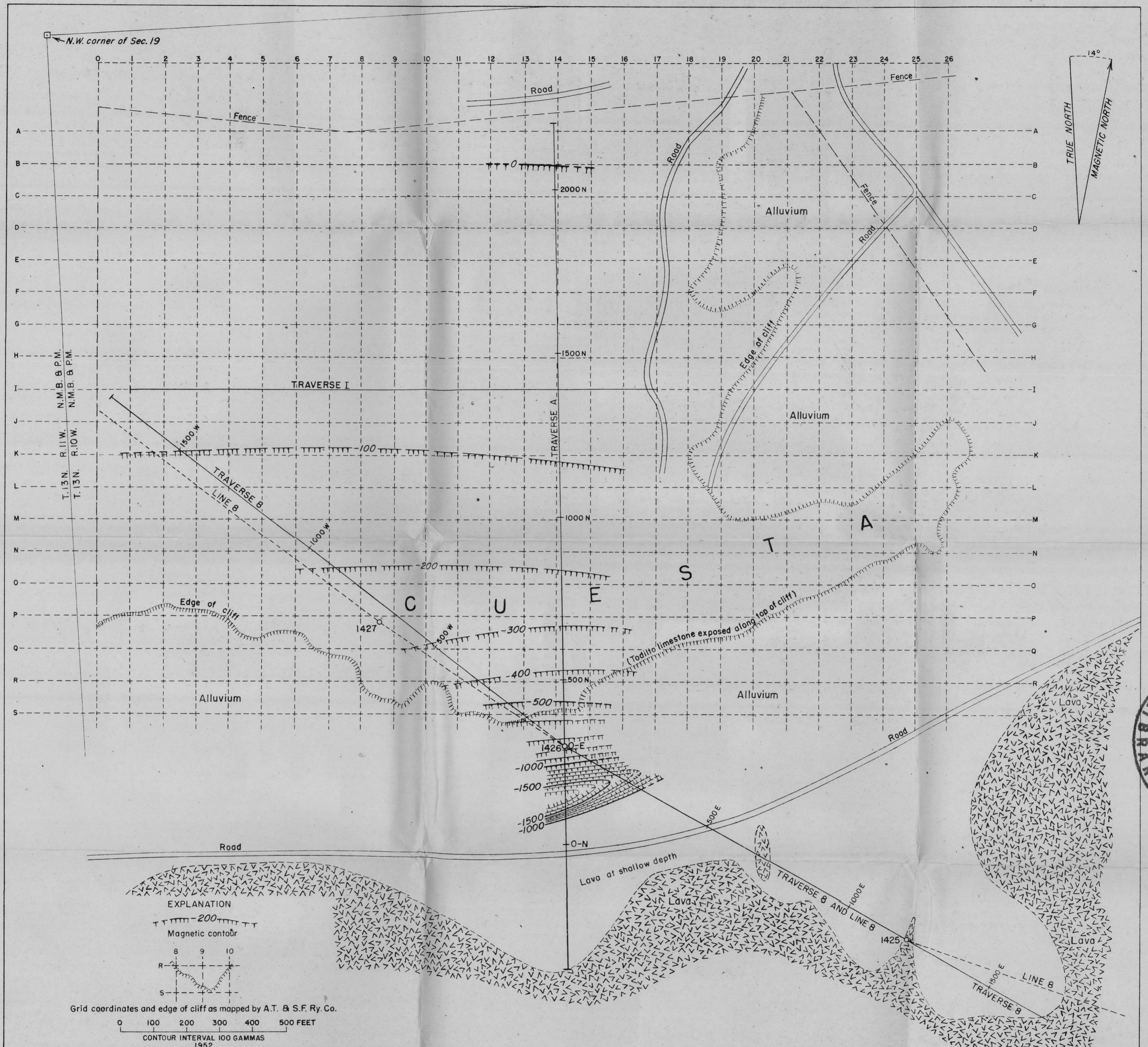
Figure 2. - Portion of Section 19, T.13N., R.10W., N.M.B. & P.M., near Grants, New Mexico.
