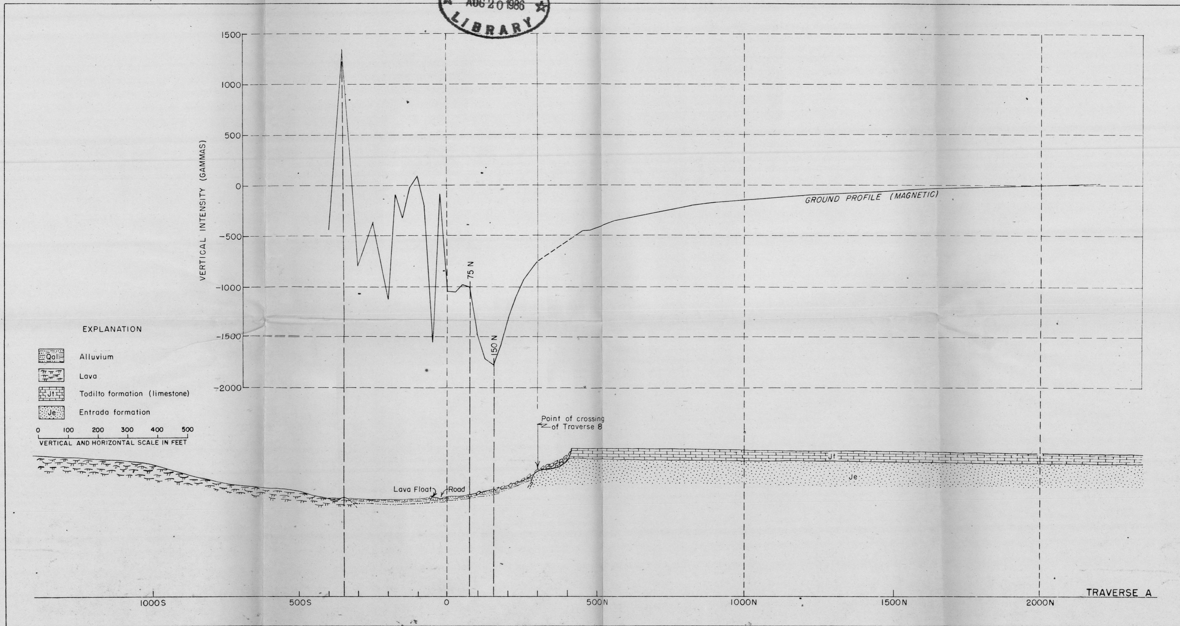
Figure 4. - Geologic cross section and magnetic profile along Traverse A.
