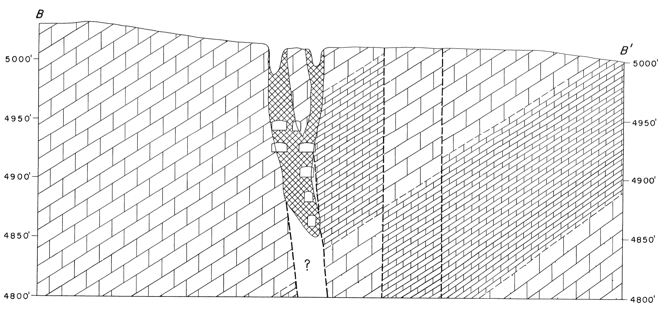
FIGURE 8. —GEOLOGIC SECTIONS OF THE LARGE PIPE ON THE BELL HILL PROPERTY
