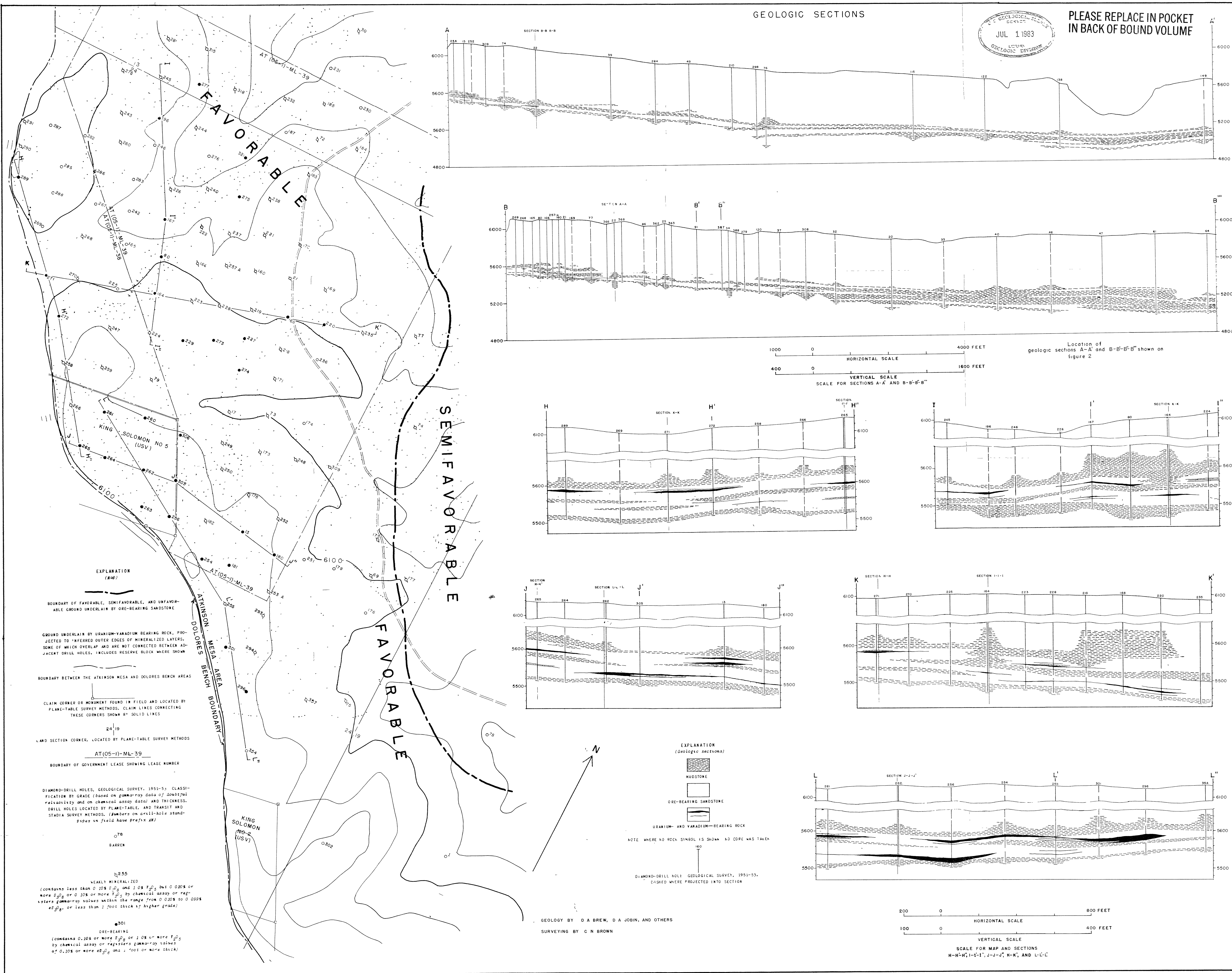
Figure 3. MAP AND GEOLOGIC SECTIONS OF THE SOUTHWESTERN PART OF ATKINSON MESA AREA, MONTROSE COUNTY, COLORADO
