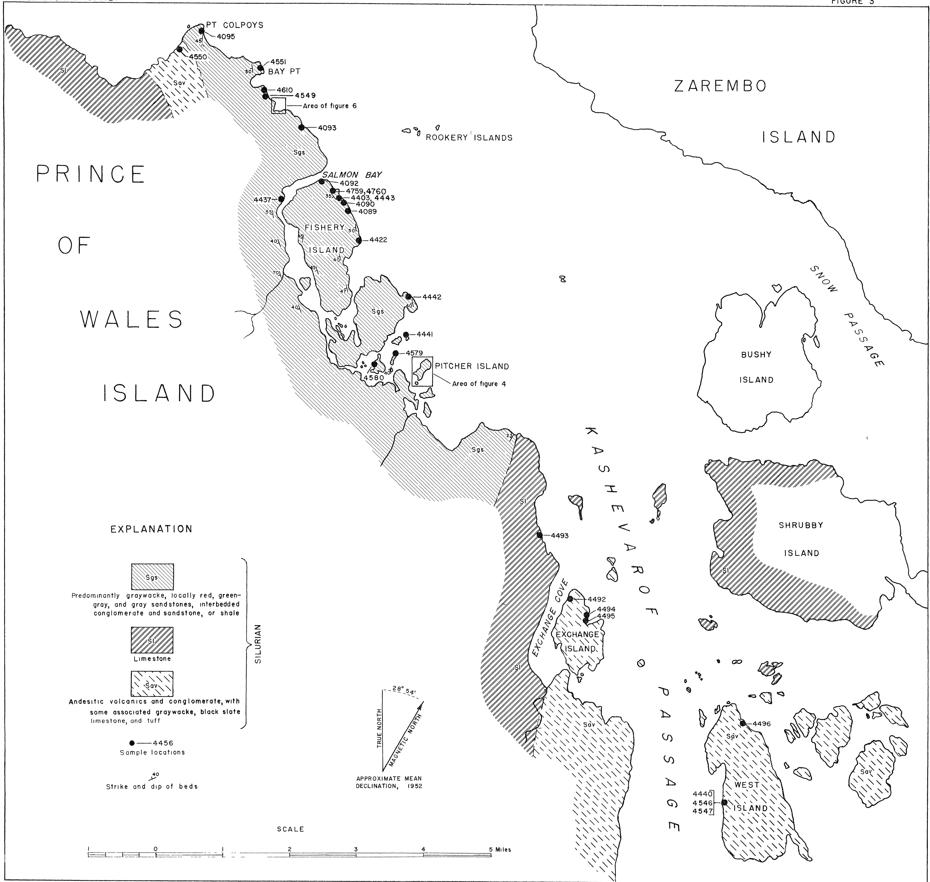
GEOLOGIC MAP OF THE SALMON BAY AREA, PETERSBURG QUADRANGLE, SOUTHEASTERN ALASKA
