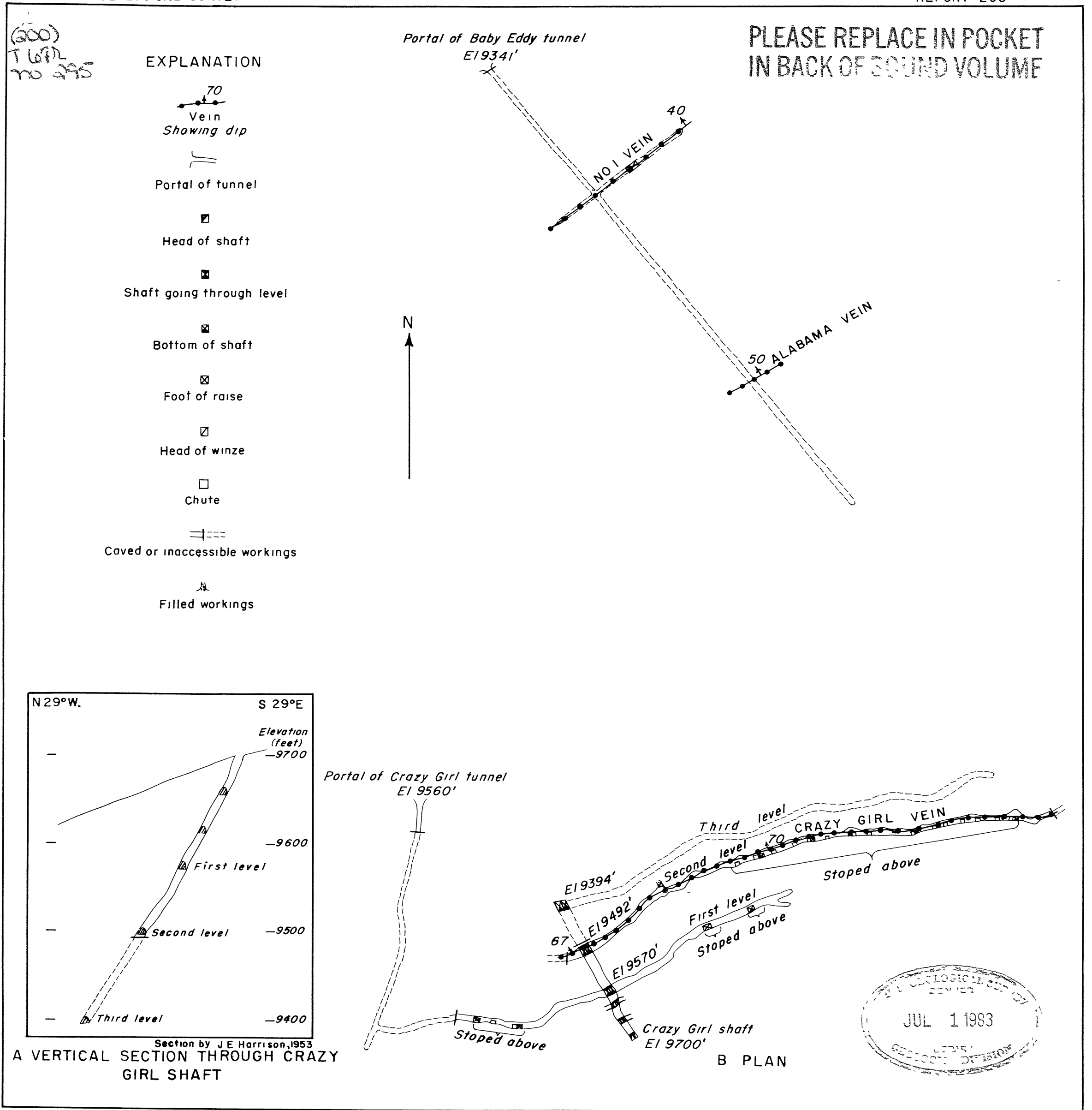
FIGURE 20.—PLAN AND SECTION OF THE CRAZY GIRL MINE, FREELAND-LAMARTINE DISTRICT, COLORADO.
