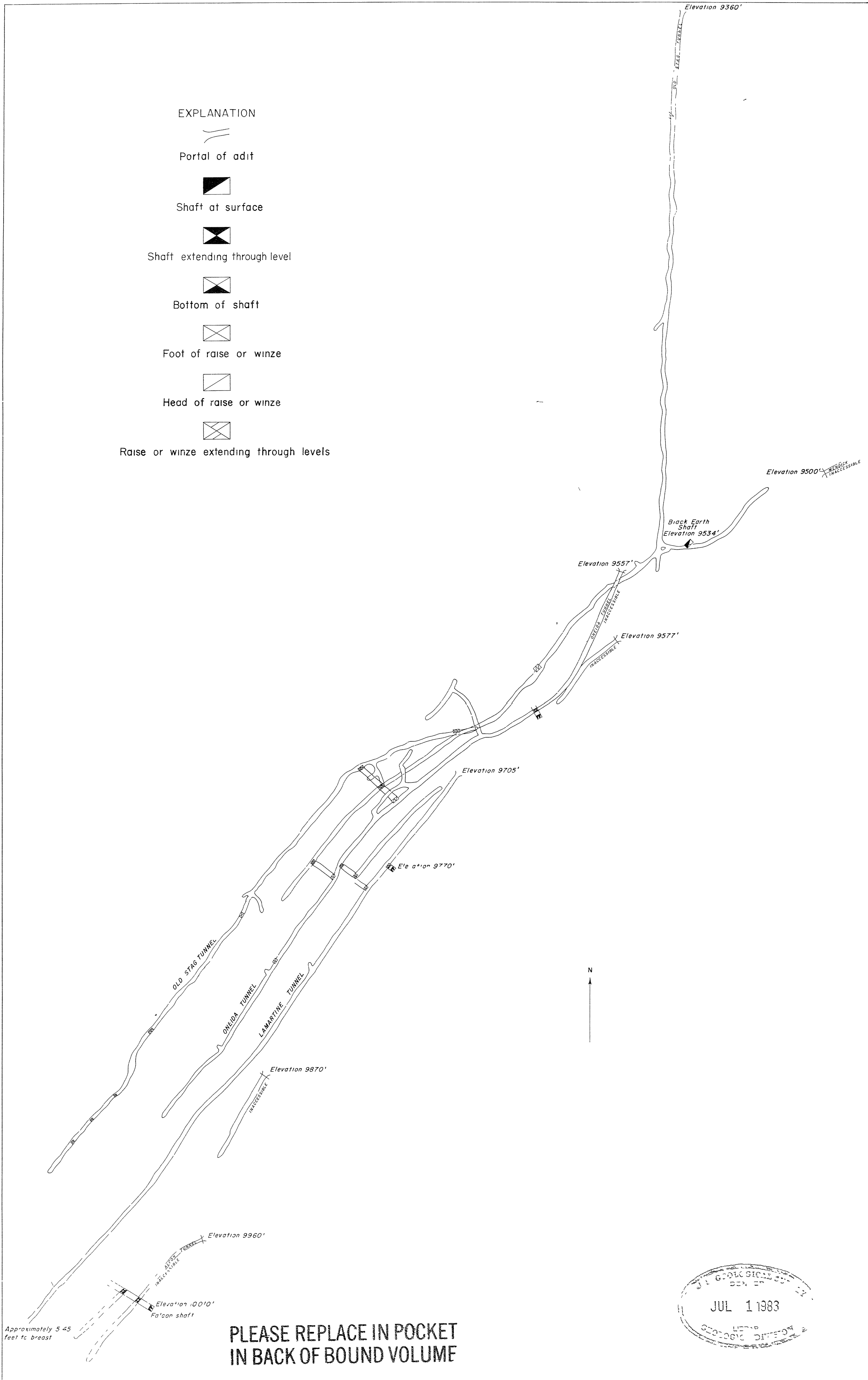
FIGURE 26-PLAN OF PART OF THE WORKINGS ON THE ONEIDA-MENDICK VEINS, FREELAND-LAMARTINE DISTRICT, COLORADO
