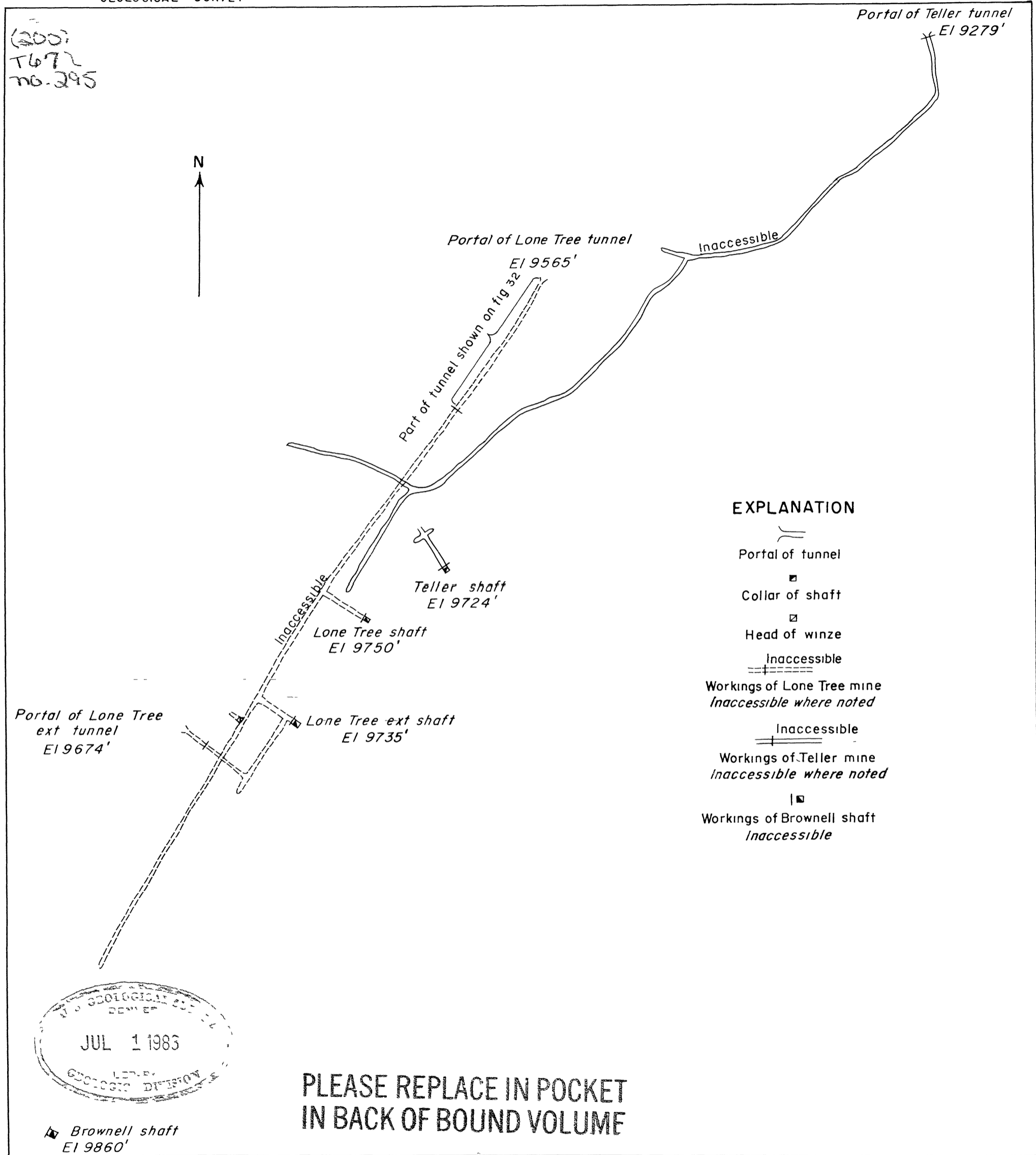
FIGURE 31-PLANS OF THE LONE TREE AND TELLER MINES, FREELAND-LAMARTINE DISTRICT, COLORADO
