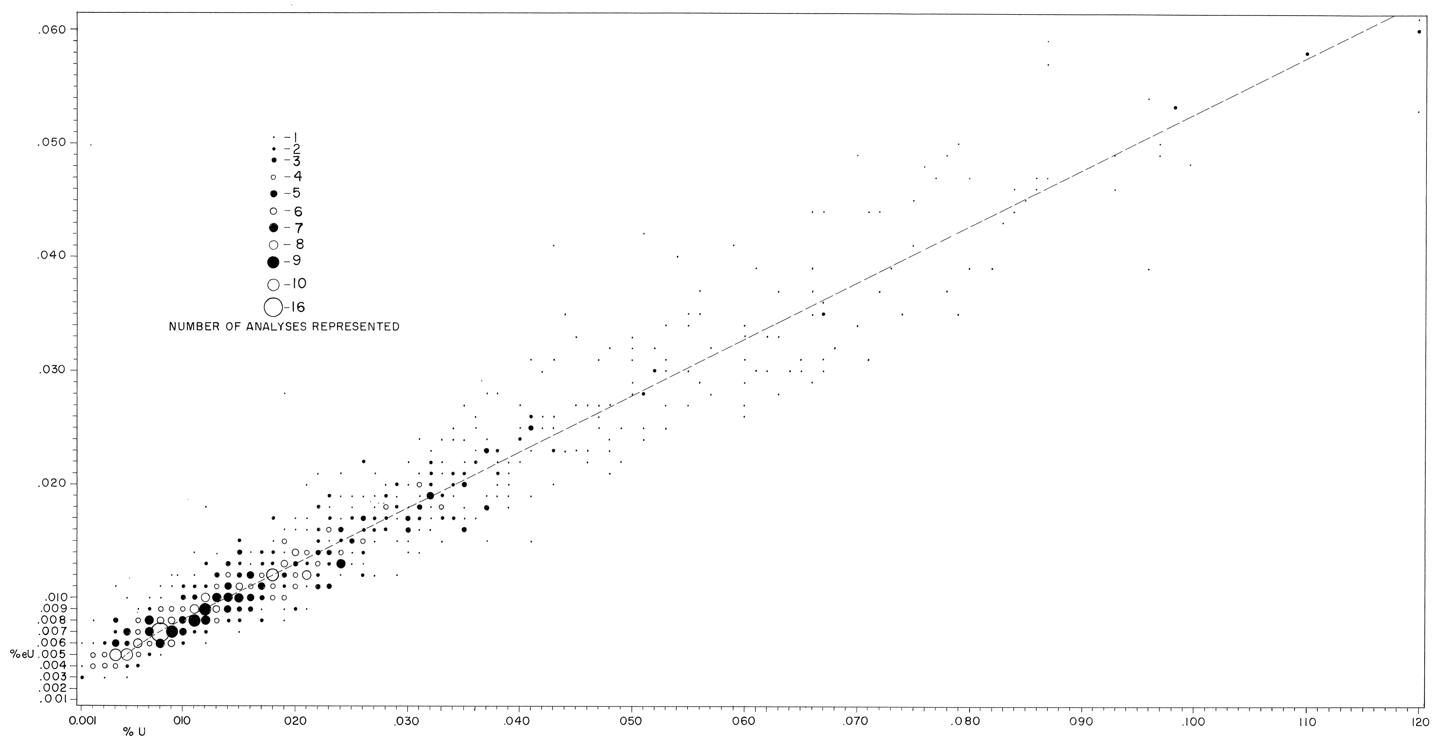
PLATE 22.—GRAPH SHOWING RELATIONSHIP OF EQUIVALENT URANIUM TO URANIUM IN THE LOST CREEK SCHROECKINGERITE DEPOSITS, ANALYSES OF 820 SAMPLES FROM TRENCHES
