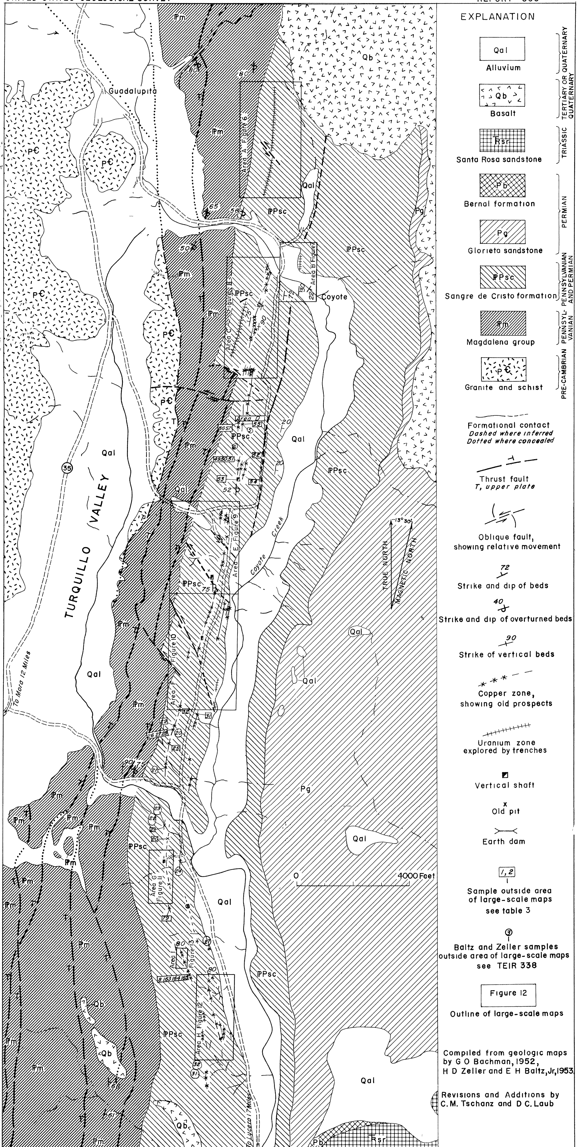
FIGURE 2.—GENERALIZED GEOLOGIC MAP OF THE COYOTE DISTRICT, MORA COUNTY, NEW MEXICO
