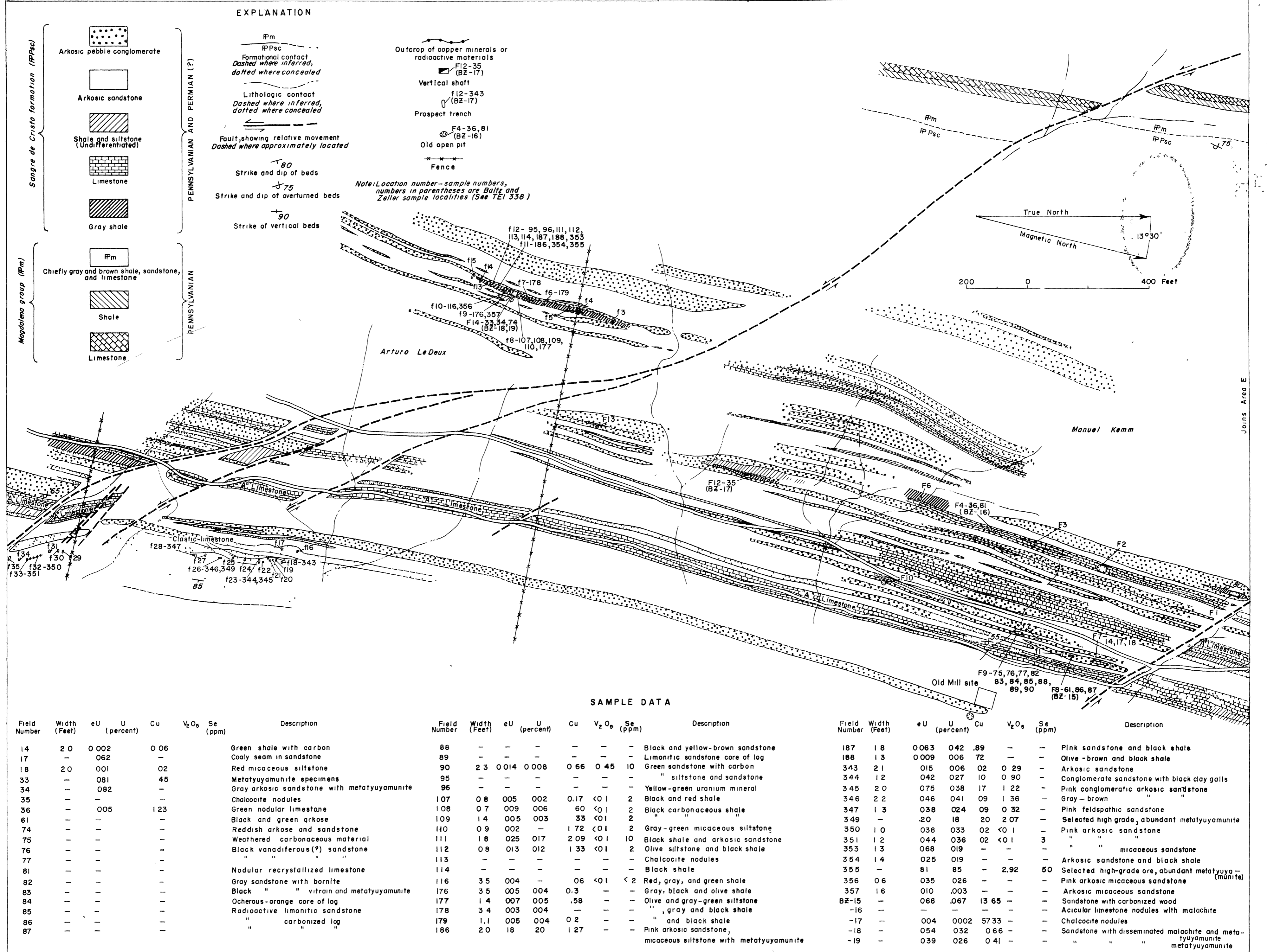
FIGURE 10. — GEOLOGIC MAP OF AREA F SHOWING COPPER AND URANIUM DEPOSITS, COYOTE DISTRICT, MORA COUNTY, NEW MEXICO
