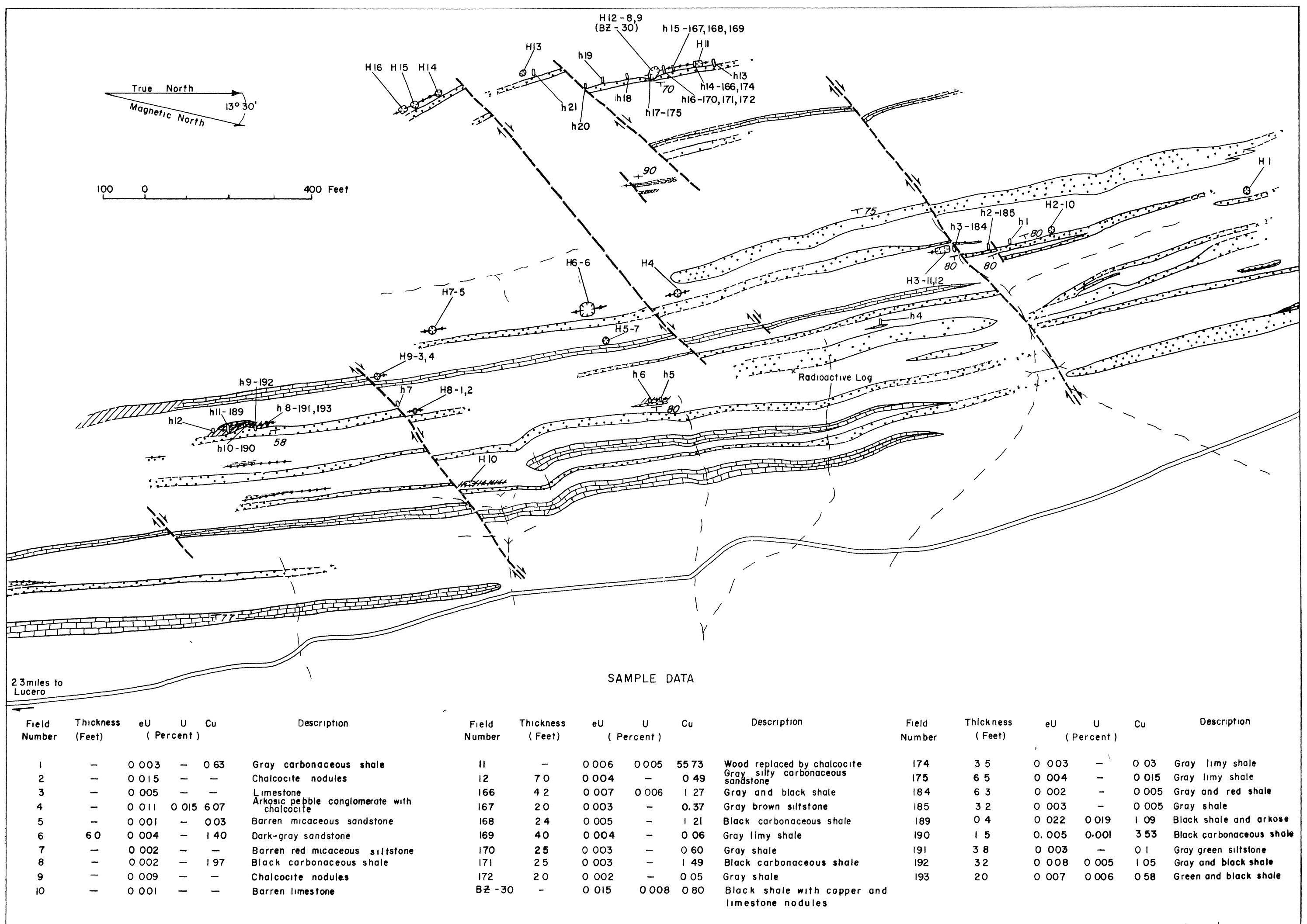
FIGURE III - GEOLOGIC MAP OF AREA H SHOWING COPPER DEPOSITS COYOTE DISTRICT, MORA COUNTY, NEW MEXICO
