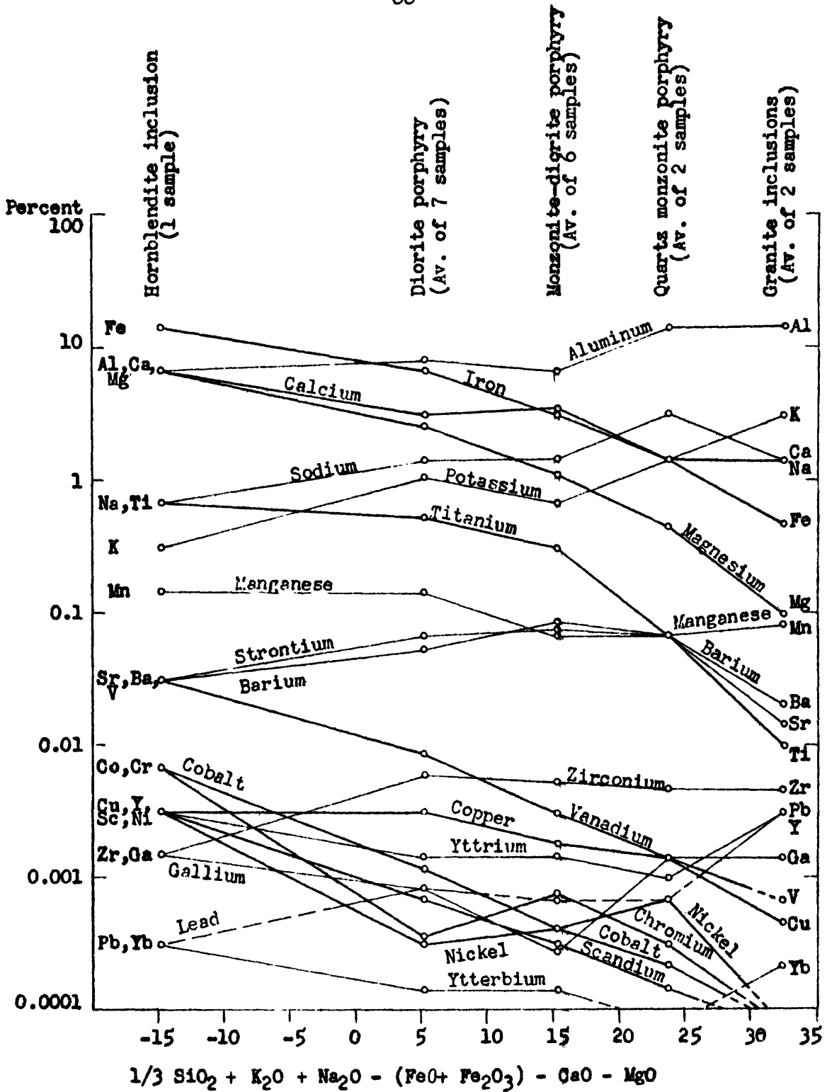
Figure 8. Variation diagram of elements, as determined spectrographically, in the igneous rocks of the Ute Mountains, Colorado
