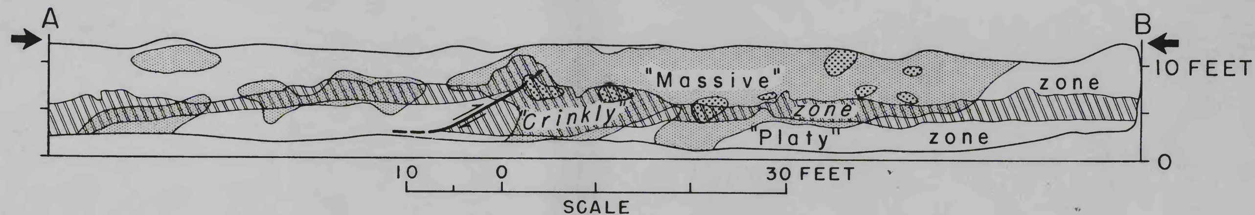
Geologic profile of west wall of crosscut
