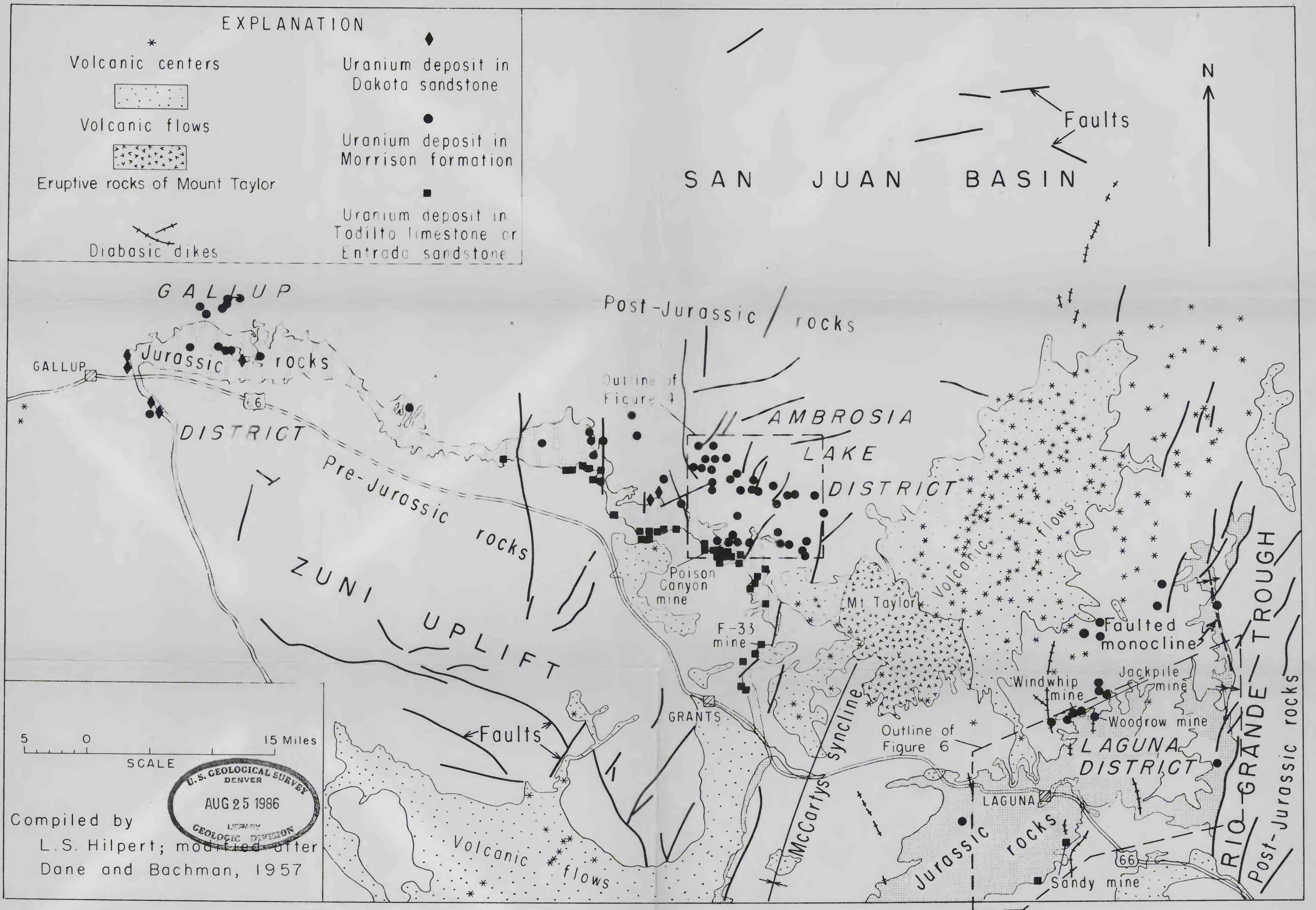
Figure 2.--Geologic map of the southern part of the San Juan Basin and vicinity showing the uranium deposits and outline of figures 4 and 6.
