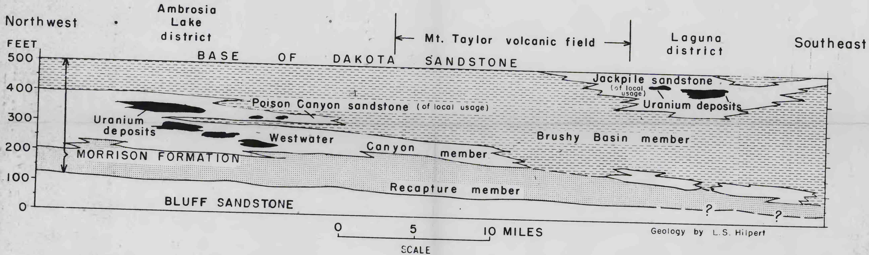
Figure 3.--Diagrammatic geologic section showing the uranium deposits and stratigraphic relations of the Morrison formation between the Ambrosia Lake and Laguna districts, New Mexico.
