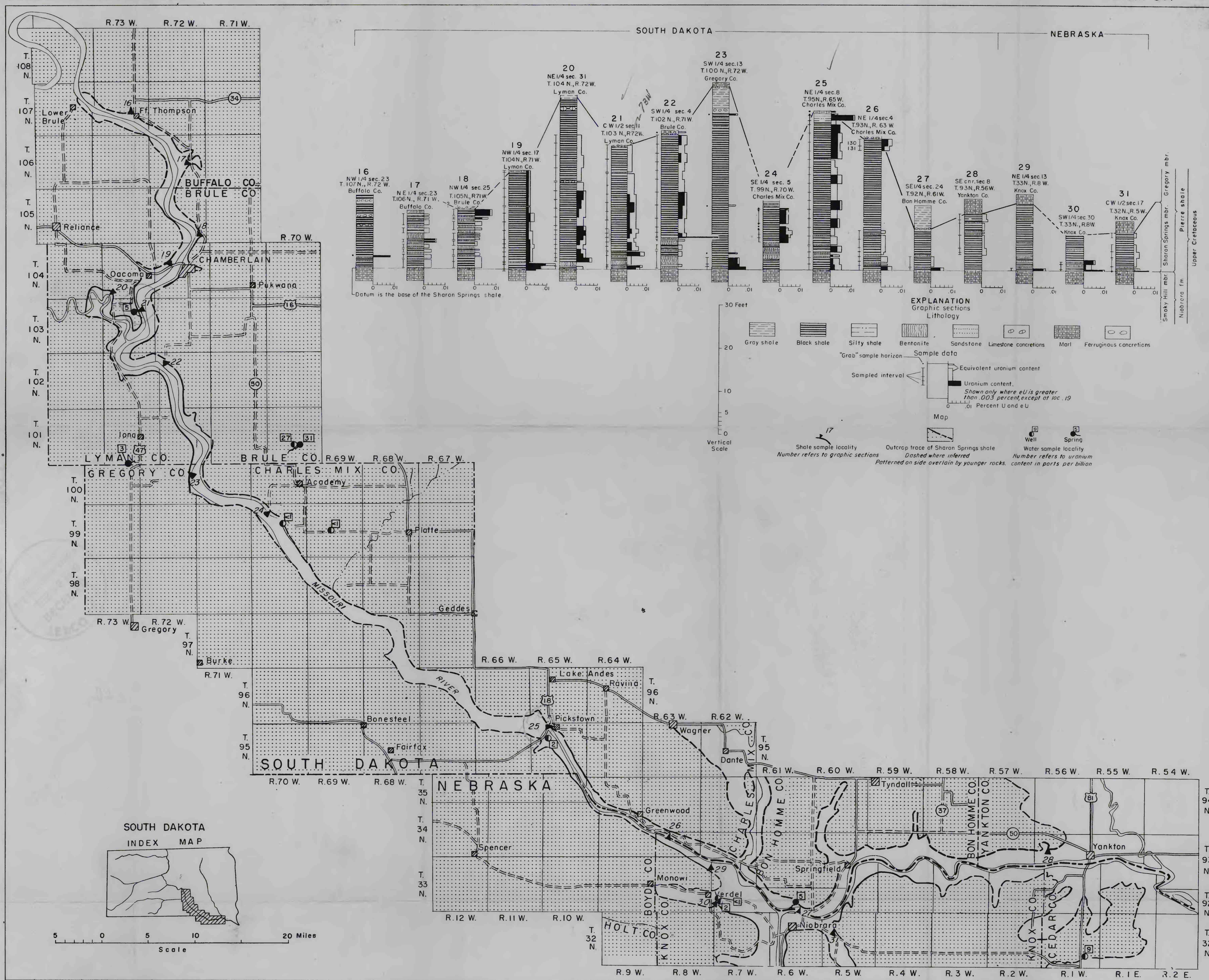
PLATE I.—OUTCROP MAP AND GRAPHIC SECTIONS SHOWING SAMPLE LOCALITIES AND URANIUM CONTENT OF THE SHARON SPRINGS MEMBER OF THE PIERRE SHALE ALONG THE MISSOURI RIVER, SOUTH DAKOTA AND NEBRASKA.
