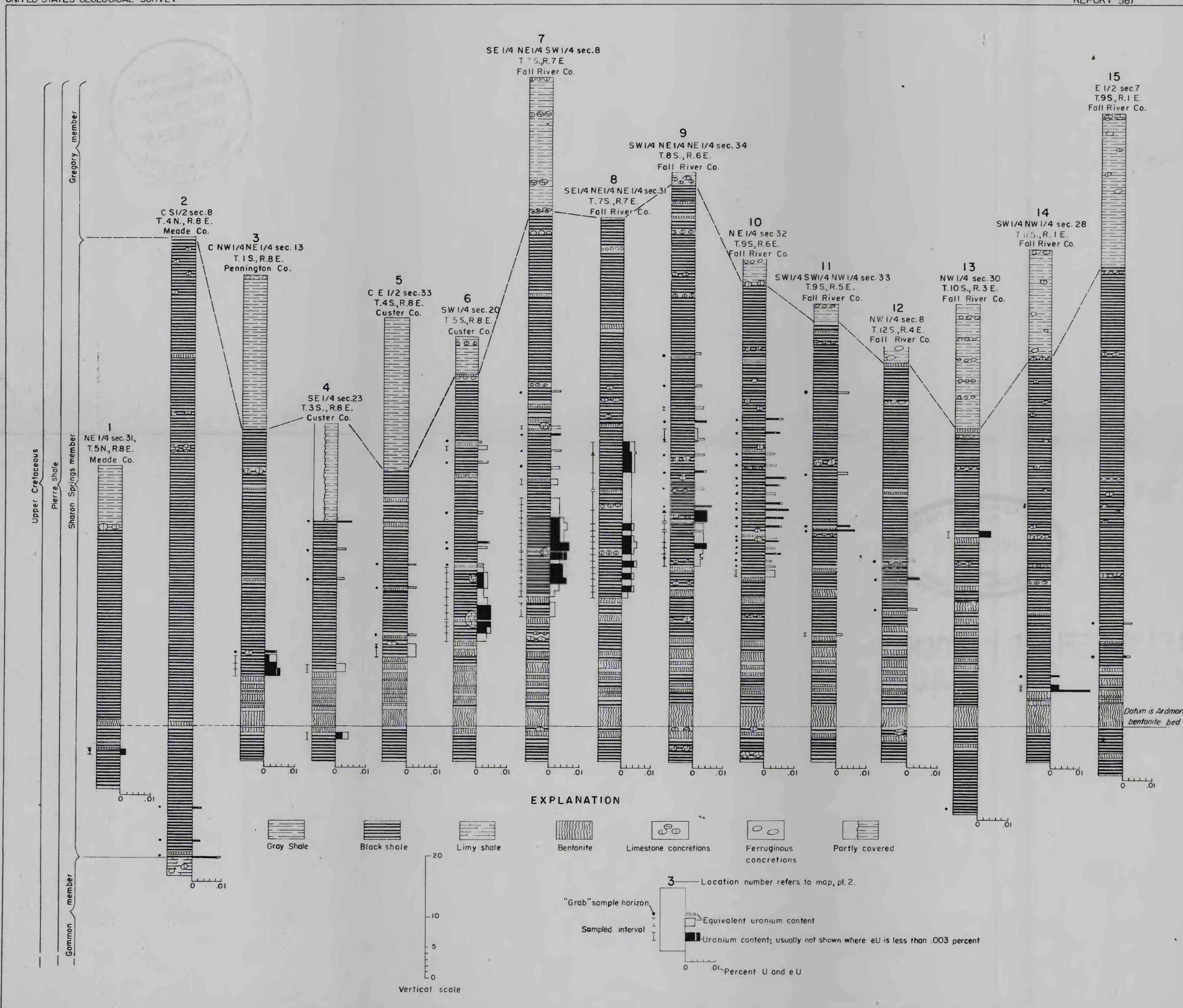
PLATE 3.—GRAPHIC SECTIONS SHOWING URANIUM CONTENT OF SHARON SPRINGS MEMBER OF PIERRE SHALE ALONG THE EASTERN AND SOUTHERN FLANKS OF THE BLACK HILLS, SOUTH DAKOTA.
