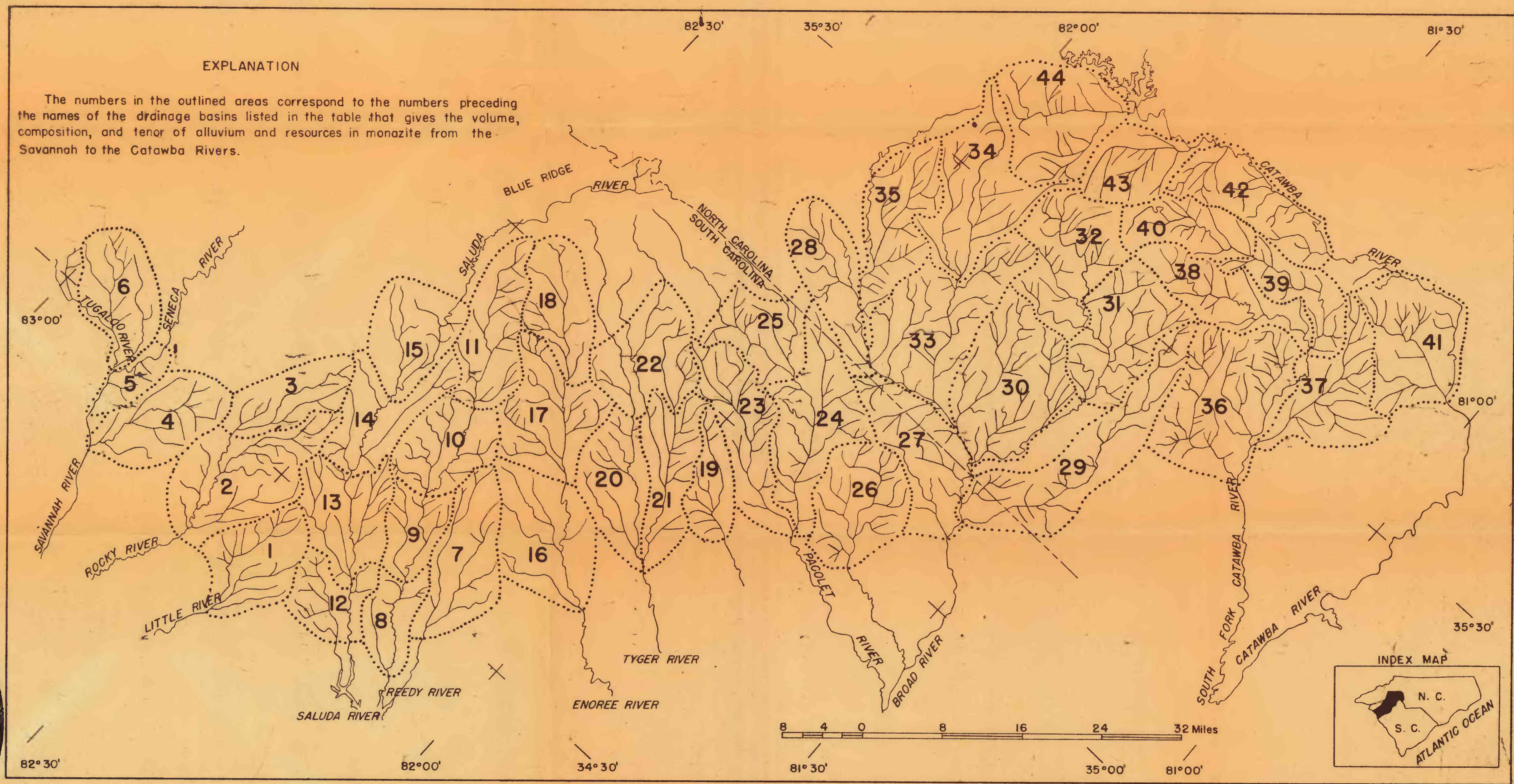
Figure 1. Map showing the locations of the 44 drainage basins appraised for placer monazite between the Savannah and Catawba Rivers, South Carolina and North Carolina.
