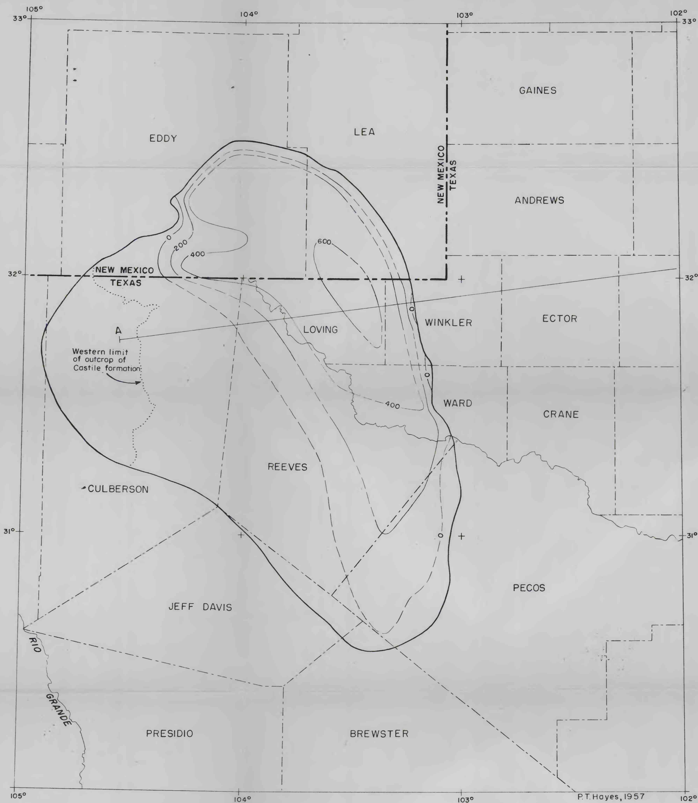
FIG. 2. MAP OF DELAWARE BASIN, NEW MEXICO AND TEXAS, SHOWING AGGREGATE THICKNESS OF SALT IN CASTILE FORMATION
