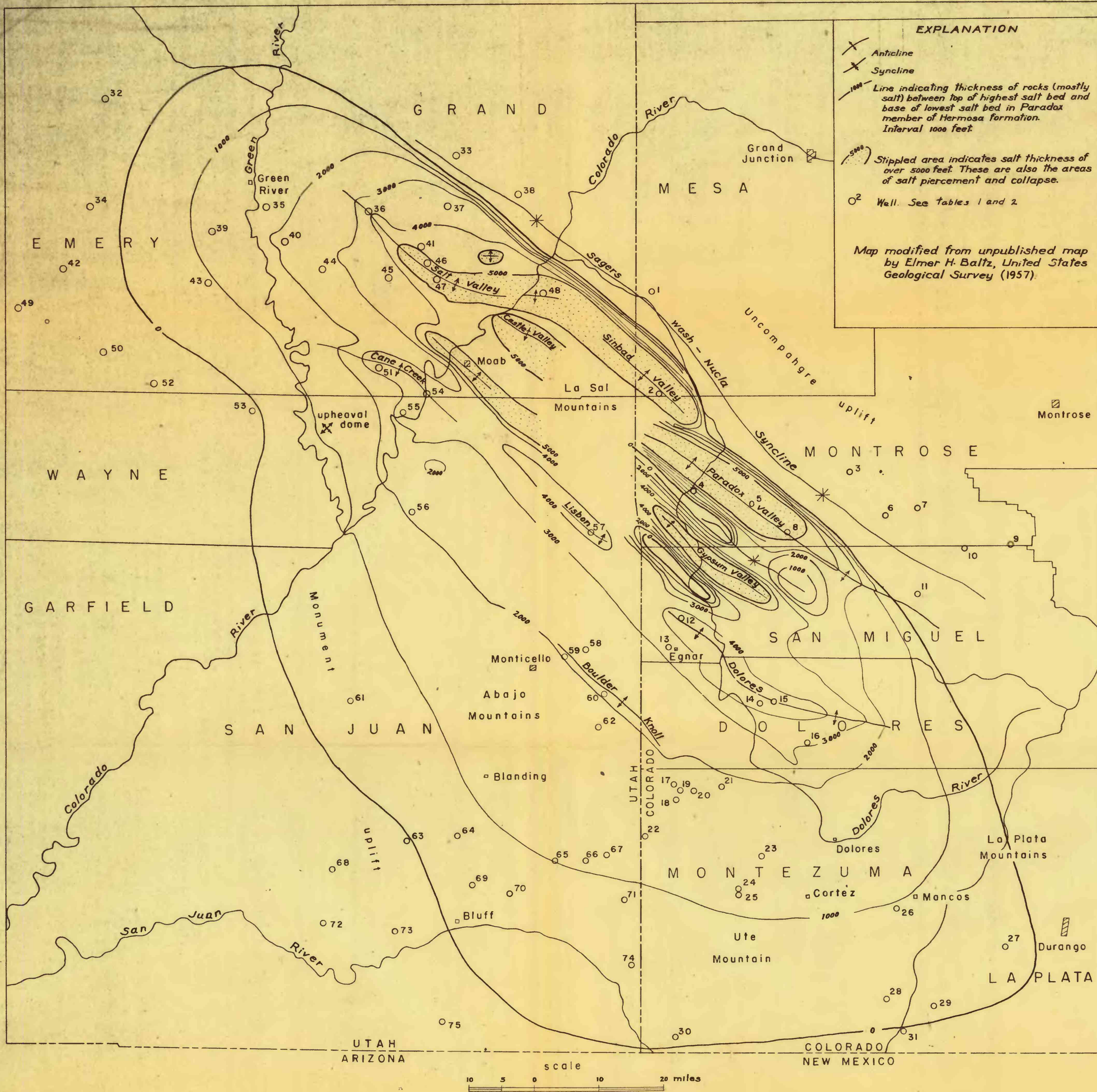
Figure 24—Map showing thickness of salt-bearing rocks of Paradox member of Hermosa formation, southeastern Utah and southwestern Colorado.
