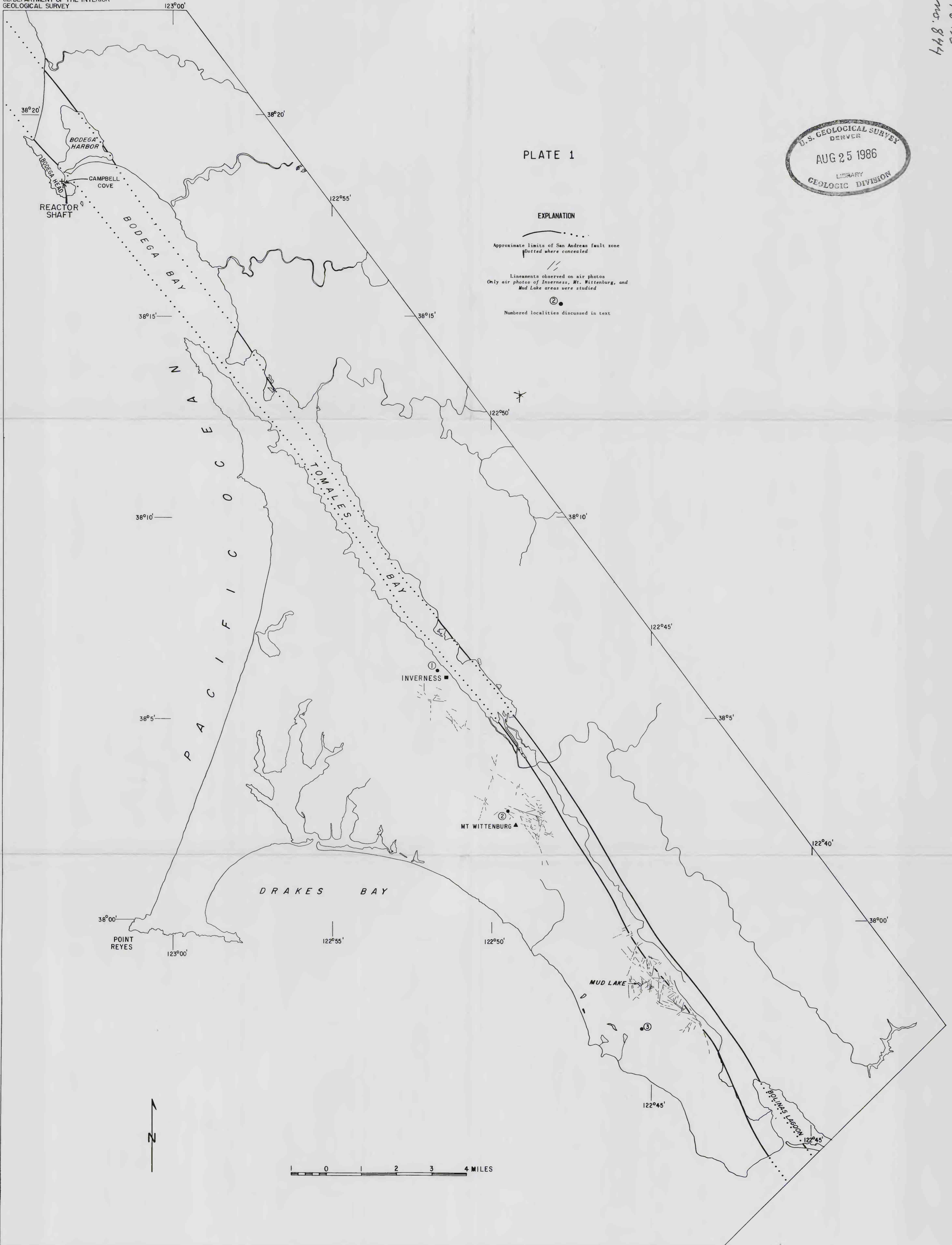
MAP SHOWING REACTOR SHAFT, SAN ANDREAS FAULT ZONE, LINEAMENTS, AND LOCALITIES DISCUSSED IN TEXT
