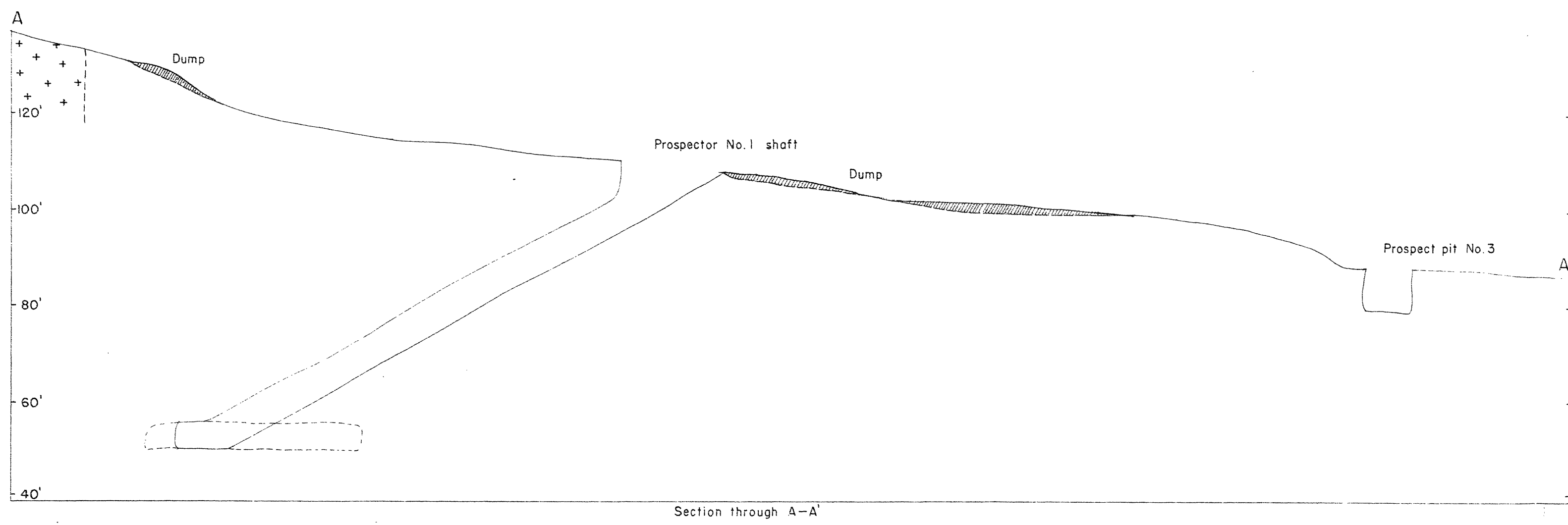
Section through A-A'
