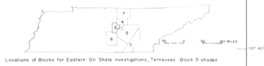
Locations of Blocks for Eastern Oil Shale investigations, Tennessee. Block 5 shaded
