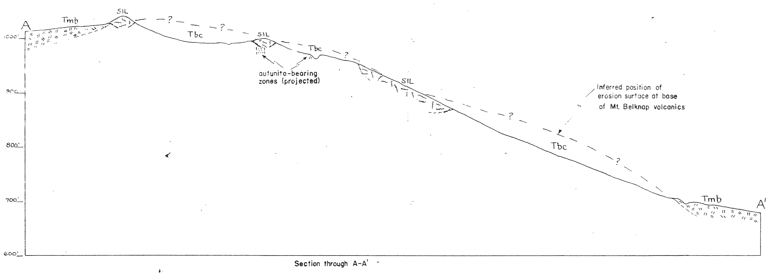
Geology and topography by E.P.Kaiser, H.L.Bauer, F.L.Klinger June 26, 1950
