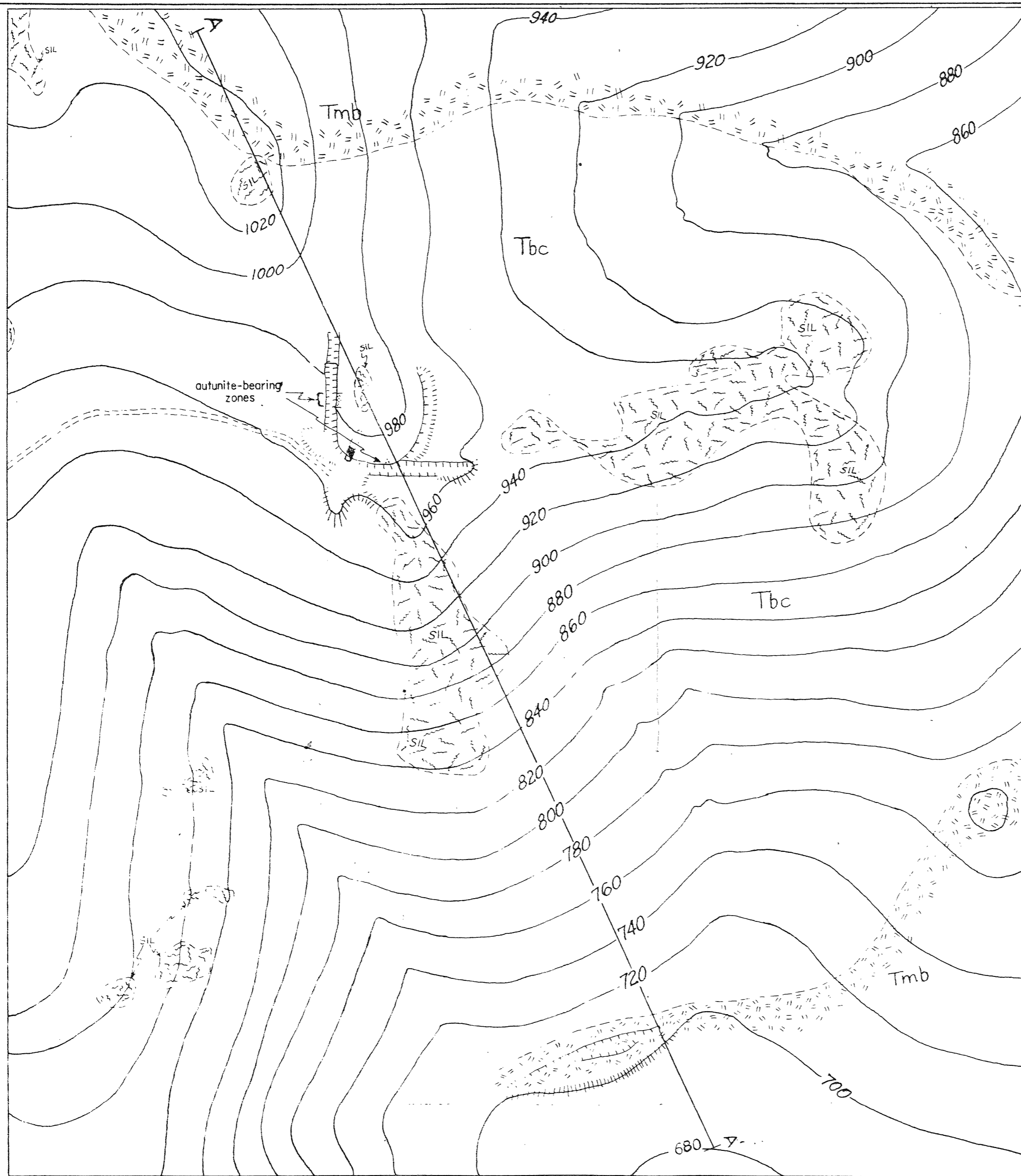
Geology and topography by E.P.Kaiser, H.L.Bauer, F.L.Klinger June 26, 1950
