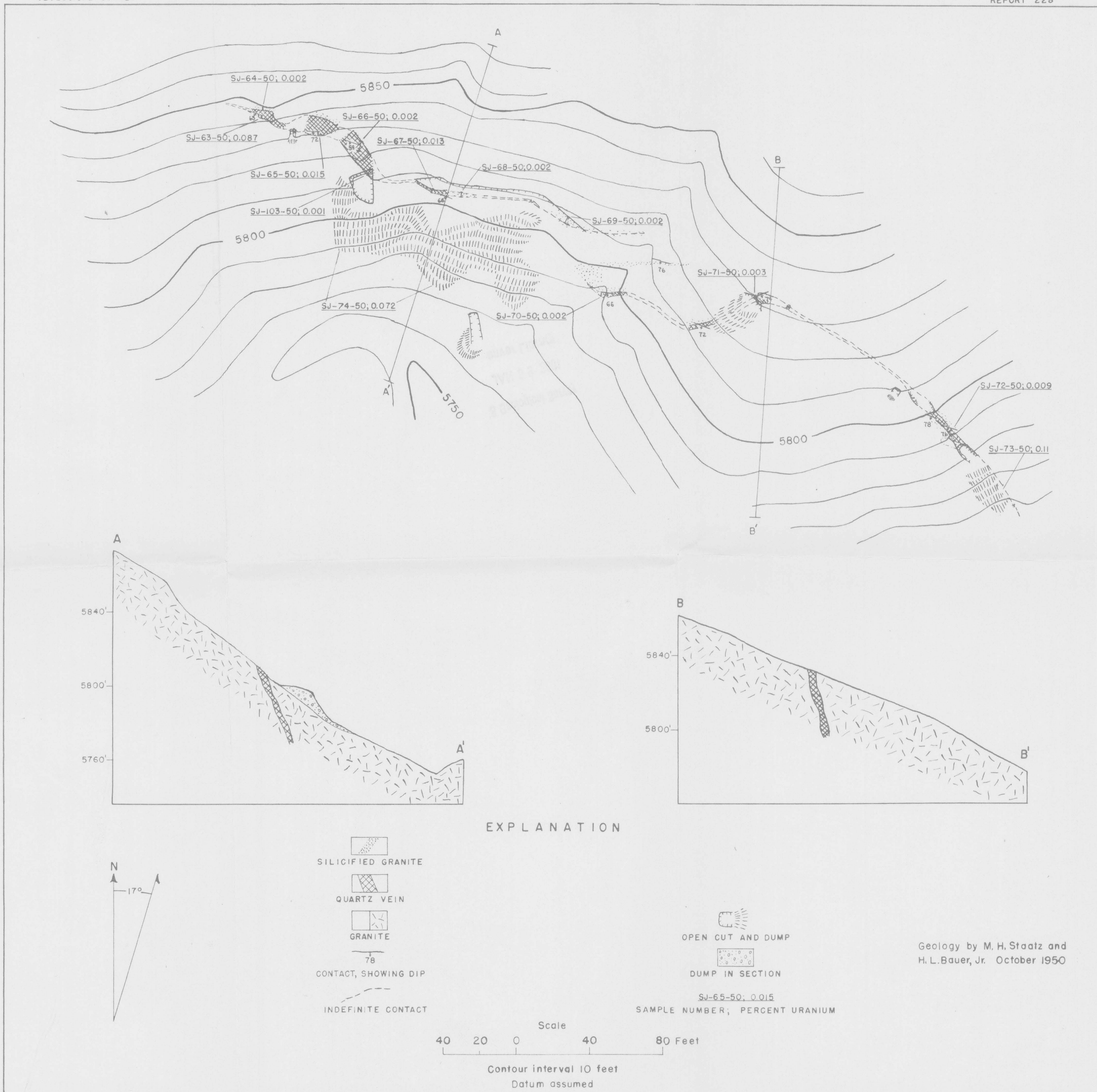
FIGURE 3. GEOLOGIC MAP AND SECTIONS OF THE WEST WILLYS CLAIM, LYON COUNTY, NEVADA
