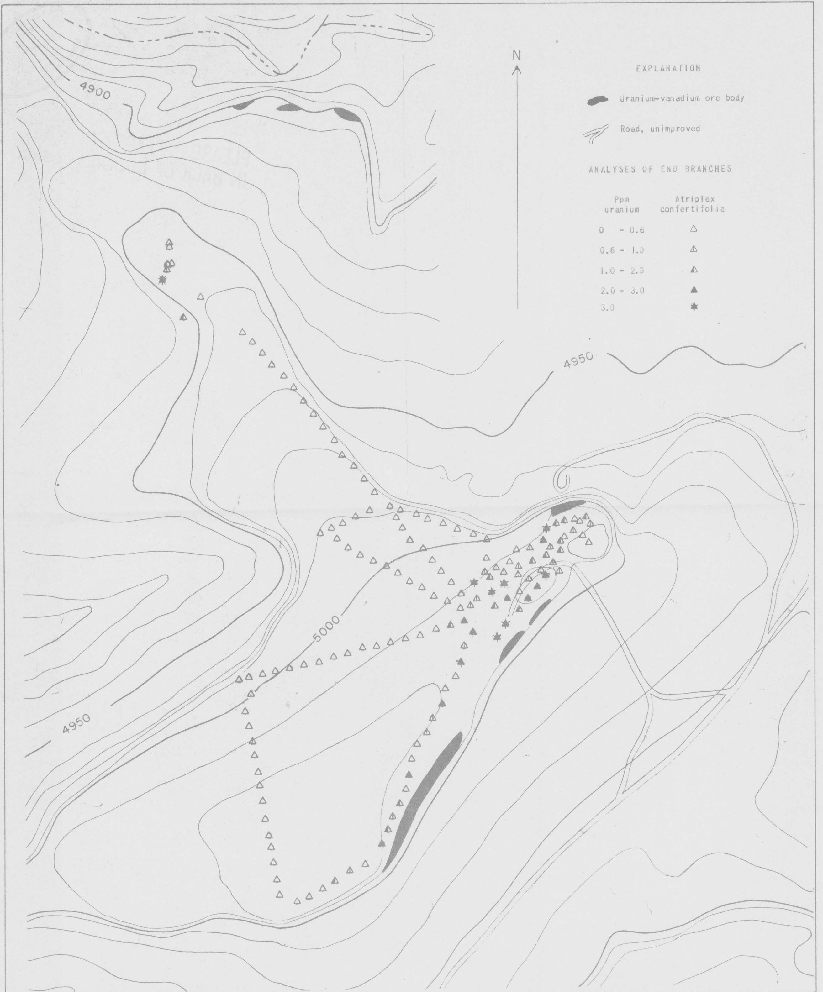
Figure 2.--Map of Yellow Cat Mesa showing uranium content of saltbush ( Atriplex confertifolia ).
