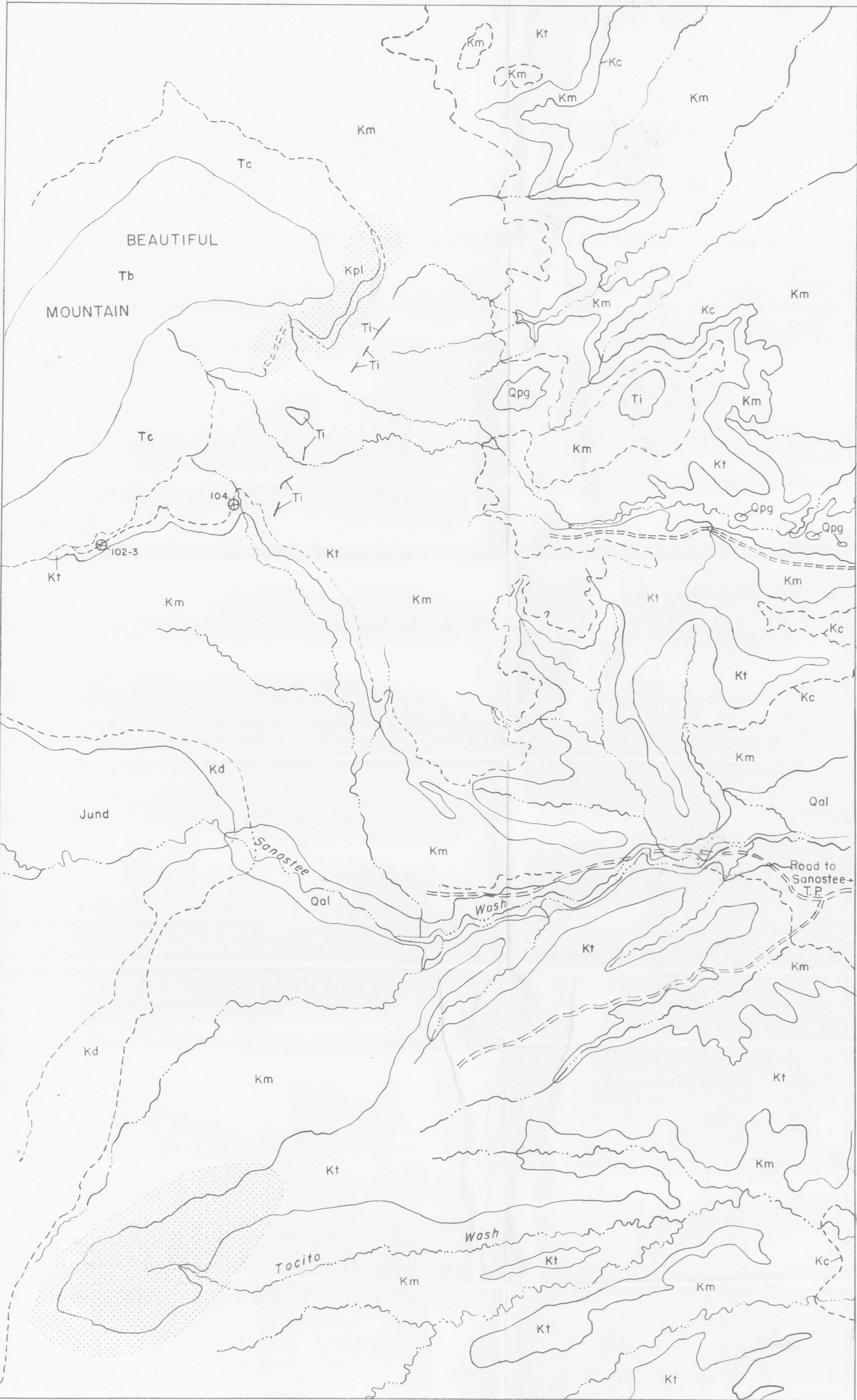
FIGURE 3. GEOLOGIC MAP OF BEAUTIFUL MOUNTAIN AND VICINITY SAN JUAN COUNTY, NEW MEXICO
