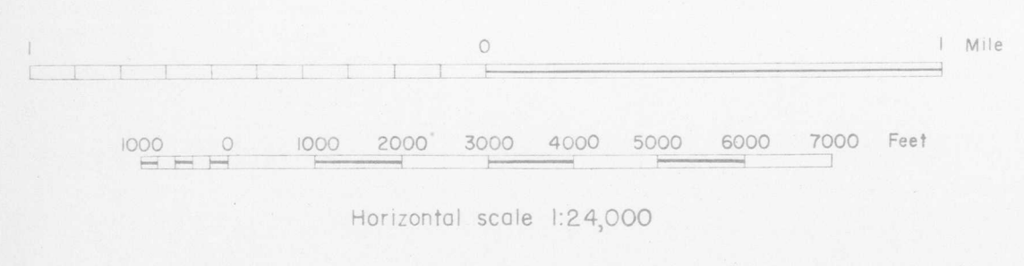
PLATE 2.— GEOLOGIC SECTIONS, PUMPKIN BUTTES AREA, CAMPBELL AND JOHNSON COUNTIES, WYOMING.
